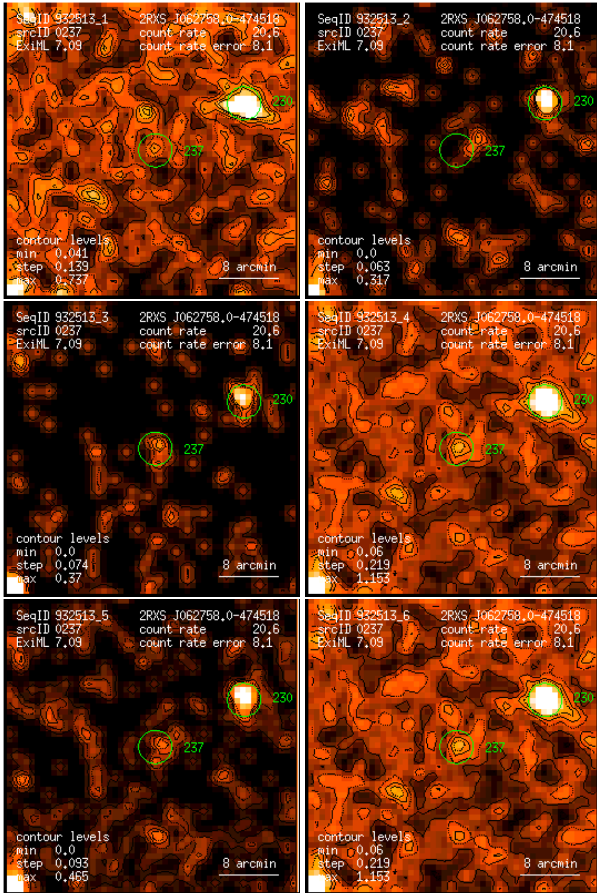
Figure 237: RASS 932513: detection 0237: band rate images, Gaussian filter: (1) PSPC channels 11 – 41, (2) 52 – 90, (3) 91 – 201, (4) 11 – 235, (5) 52 – 201, (6) 11 – 201. Broad band rates in counts/ks. Band rate contour levels in counts/ks/arcmin 2 .
