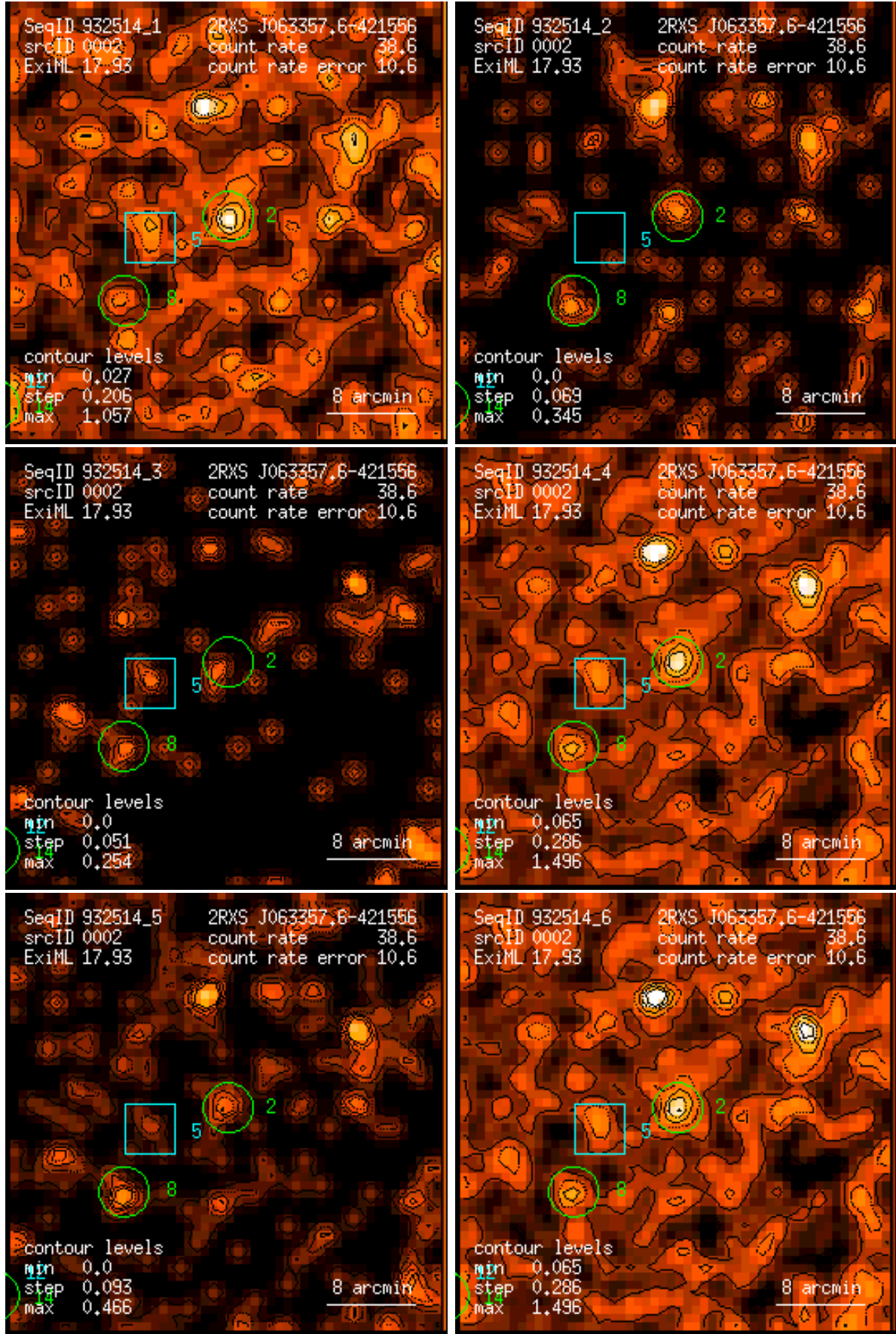
Figure 2: RASS 932514: detection 0002: band rate images, Gaussian filter: (1) PSPC channels 11 – 41, (2) 52 – 90, (3) 91 – 201, (4) 11 – 235, (5) 52 – 201, (6) 11 – 201. Broad band rates in counts/ks. Band rate contour levels in counts/ks/arcmin 2 .
