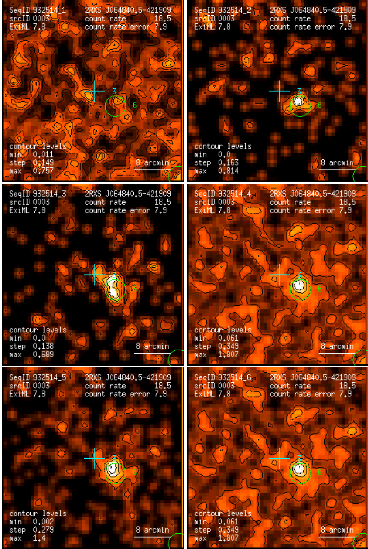
Figure 3: RASS 932514: detection 0003: band rate images, Gaussian filter: (1) PSPC channels 11 – 41, (2) 52 – 90, (3) 91 – 201, (4) 11 – 235, (5) 52 – 201, (6) 11 – 201. Broad band rates in counts/ks. Band rate contour levels in counts/ks/arcmin 2 .
