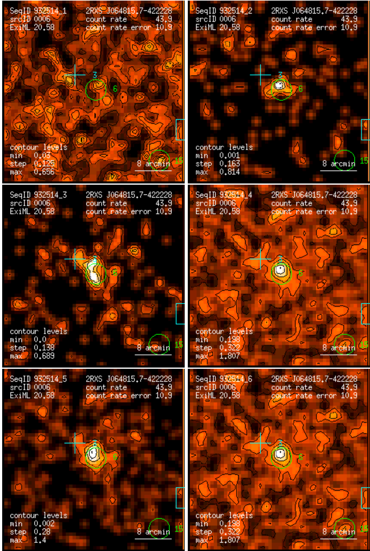
Figure 6: RASS 932514: detection 0006: band rate images, Gaussian filter: (1) PSPC channels 11 – 41, (2) 52 – 90, (3) 91 – 201, (4) 11 – 235, (5) 52 – 201, (6) 11 – 201. Broad band rates in counts/ks. Band rate contour levels in counts/ks/arcmin 2 .
