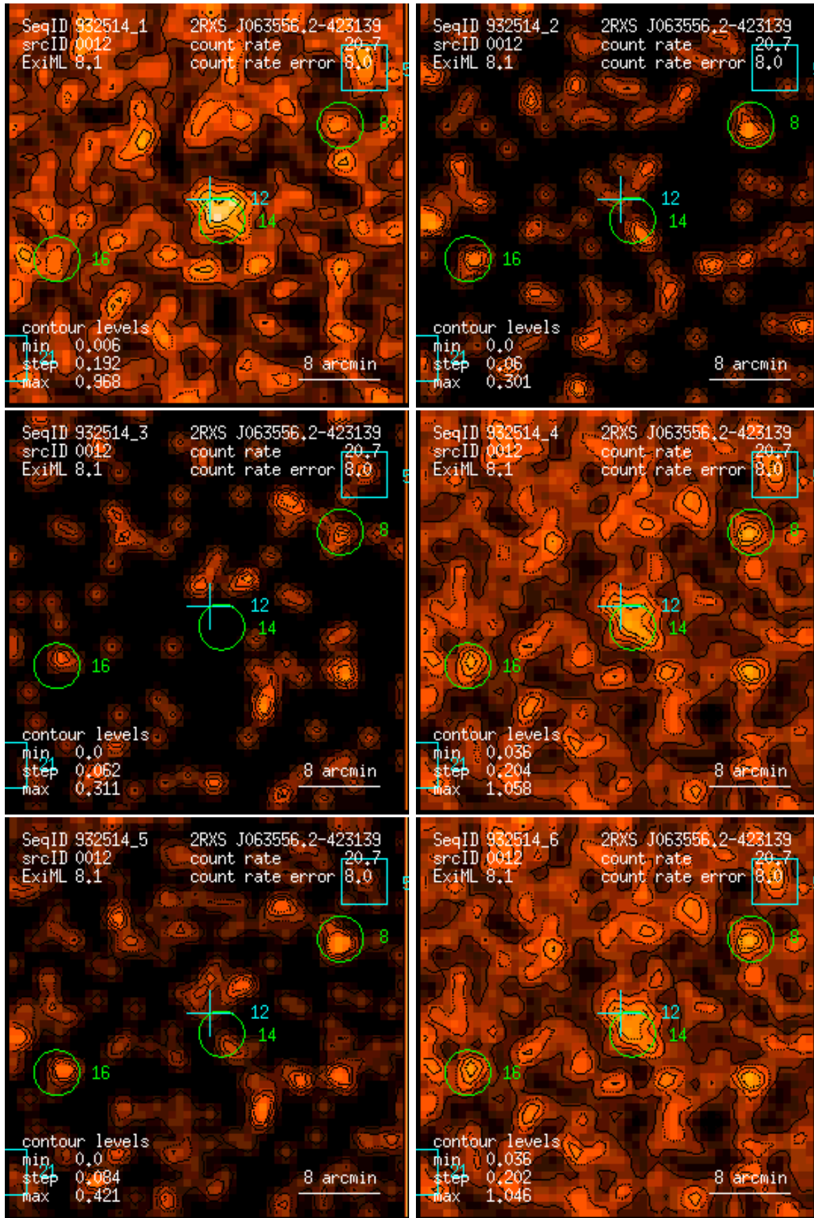
Figure 12: RASS 932514: detection 0012: band rate images, Gaussian filter: (1) PSPC channels 11 – 41, (2) 52 – 90, (3) 91 – 201, (4) 11 – 235, (5) 52 – 201, (6) 11 – 201. Broad band rates in counts/ks. Band rate contour levels in counts/ks/arcmin 2 .
