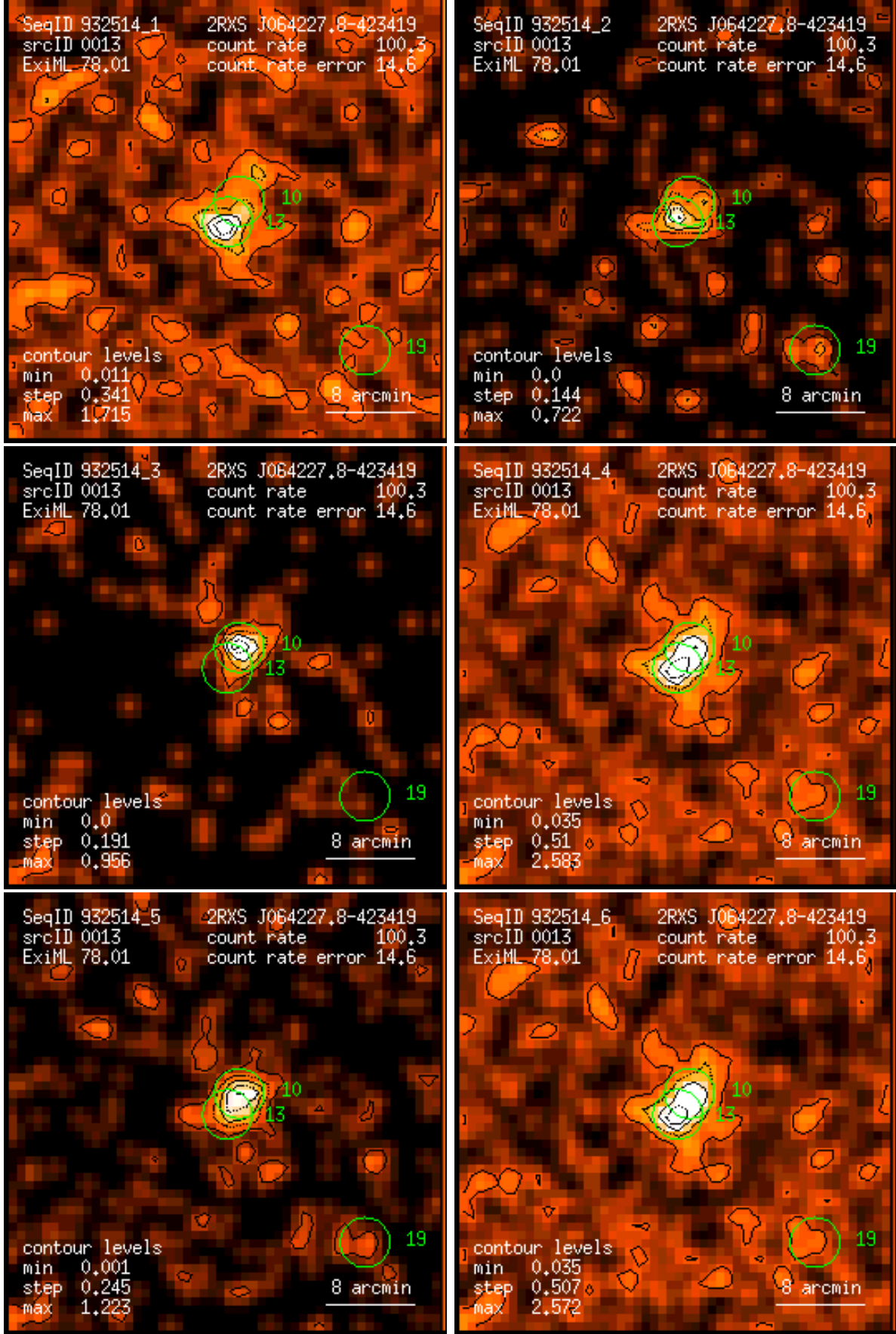
Figure 13: RASS 932514: detection 0013: band rate images, Gaussian filter: (1) PSPC channels 11 – 41, (2) 52 – 90, (3) 91 – 201, (4) 11 – 235, (5) 52 – 201, (6) 11 – 201. Broad band rates in counts/ks. Band rate contour levels in counts/ks/arcmin 2 .
