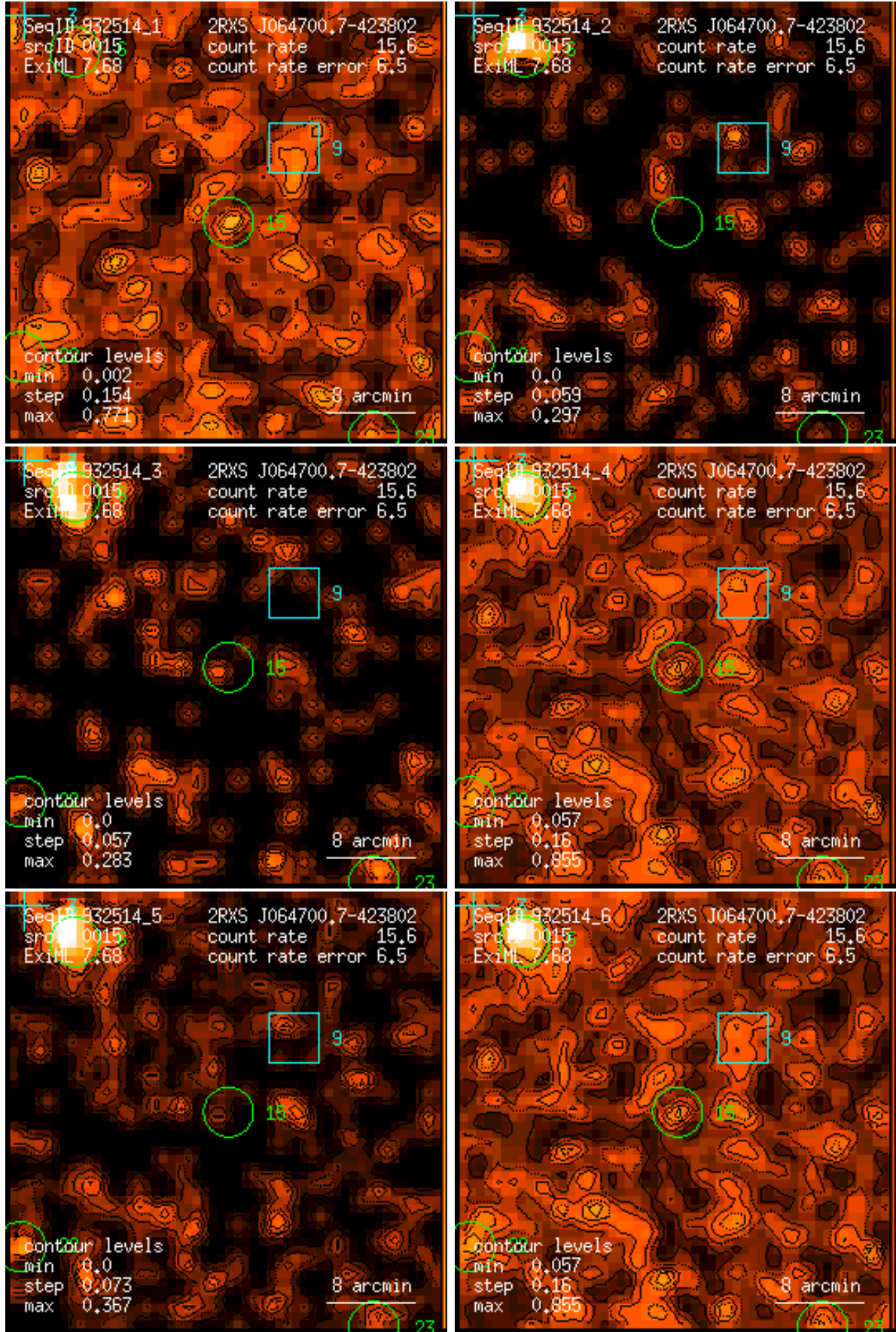
Figure 15: RASS 932514: detection 0015: band rate images, Gaussian filter: (1) PSPC channels 11 – 41, (2) 52 – 90, (3) 91 – 201, (4) 11 – 235, (5) 52 – 201, (6) 11 – 201. Broad band rates in counts/ks. Band rate contour levels in counts/ks/arcmin 2 .
