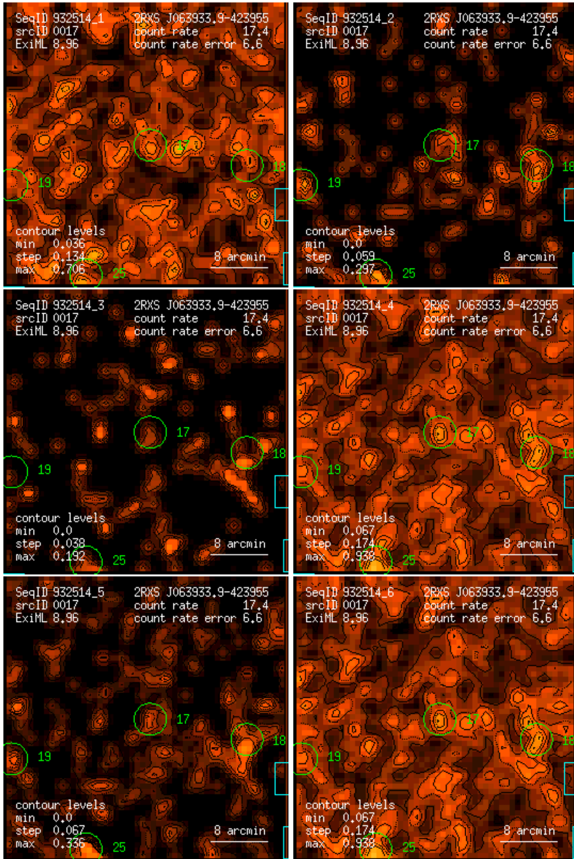
Figure 17: RASS 932514: detection 0017: band rate images, Gaussian filter: (1) PSPC channels 11 – 41, (2) 52 – 90, (3) 91 – 201, (4) 11 – 235, (5) 52 – 201, (6) 11 – 201. Broad band rates in counts/ks. Band rate contour levels in counts/ks/arcmin 2 .
