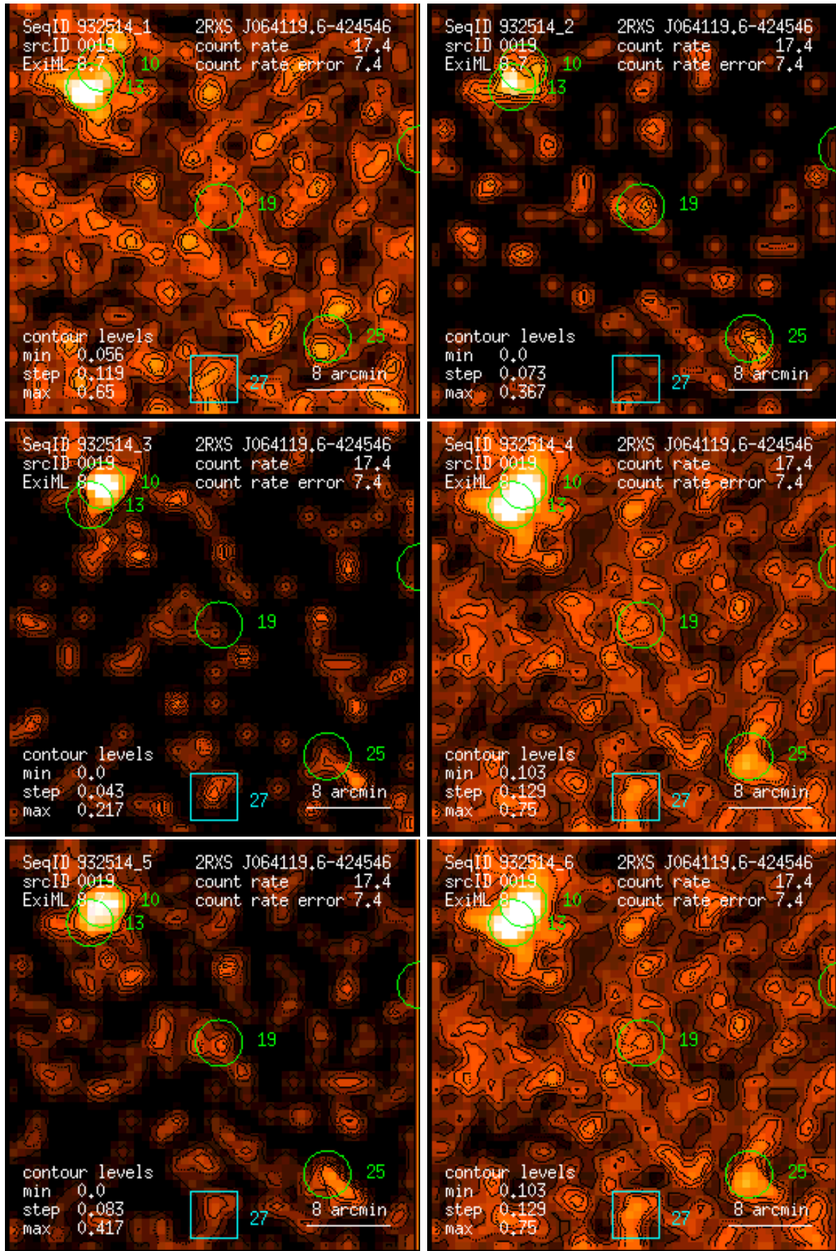
Figure 19: RASS 932514: detection 0019: band rate images, Gaussian filter: (1) PSPC channels 11 – 41, (2) 52 – 90, (3) 91 – 201, (4) 11 – 235, (5) 52 – 201, (6) 11 – 201. Broad band rates in counts/ks. Band rate contour levels in counts/ks/arcmin 2 .
