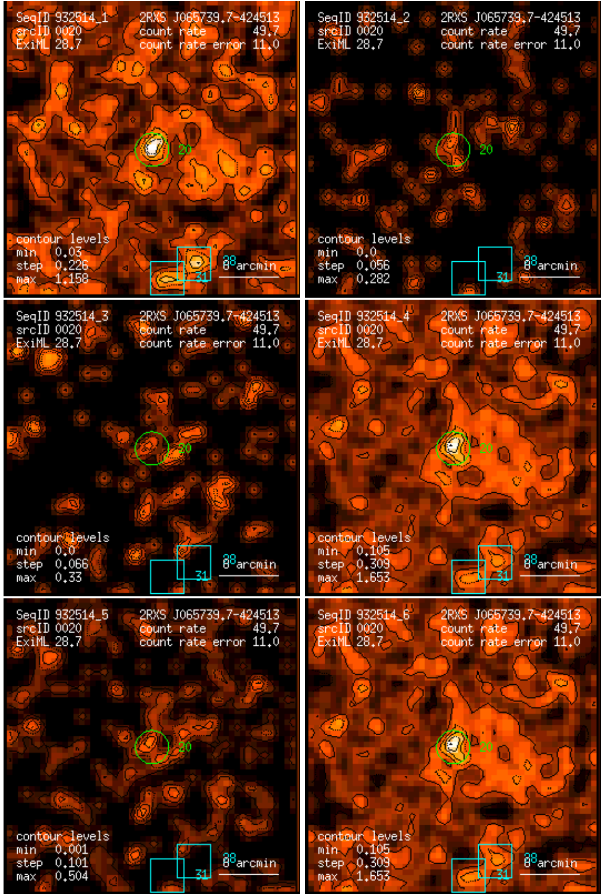
Figure 20: RASS 932514: detection 0020: band rate images, Gaussian filter: (1) PSPC channels 11 – 41, (2) 52 – 90, (3) 91 – 201, (4) 11 – 235, (5) 52 – 201, (6) 11 – 201. Broad band rates in counts/ks. Band rate contour levels in counts/ks/arcmin 2 .
