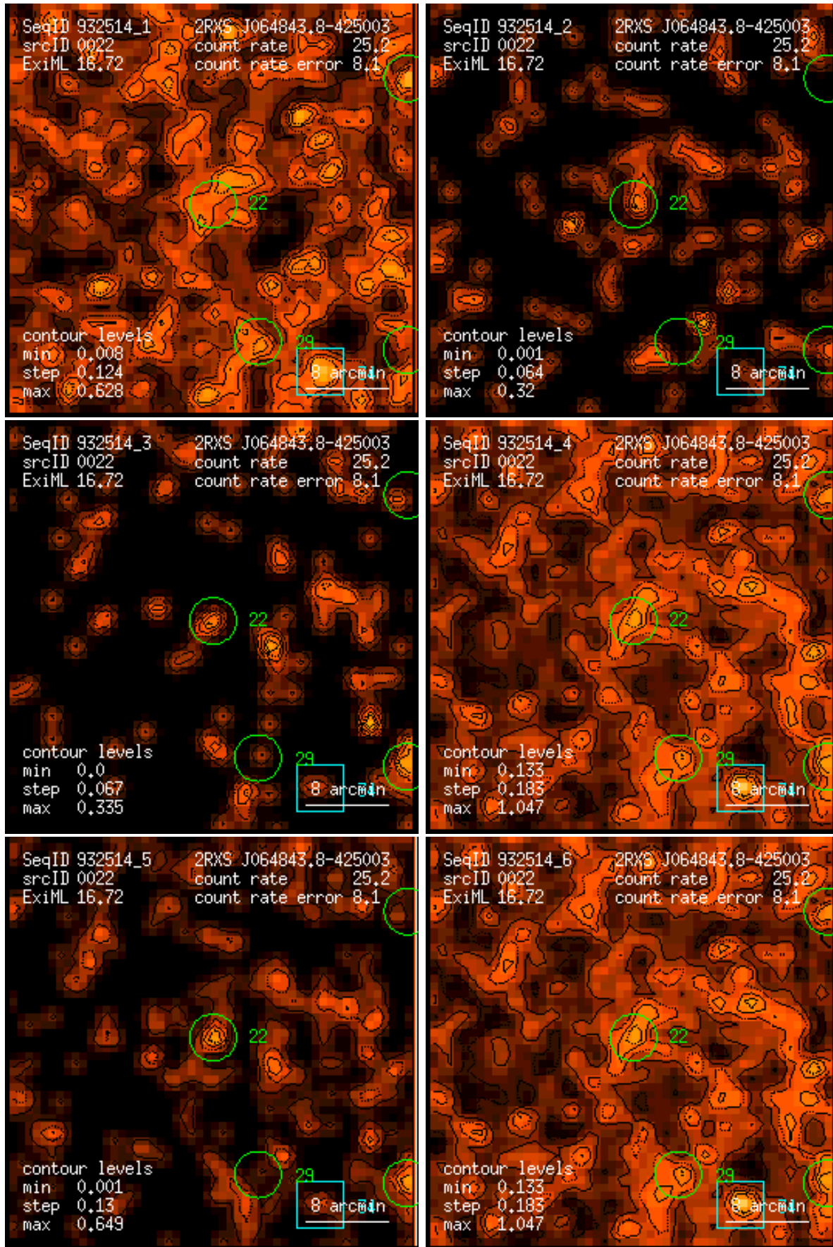
Figure 22: RASS 932514: detection 0022: band rate images, Gaussian filter: (1) PSPC channels 11 – 41, (2) 52 – 90, (3) 91 – 201, (4) 11 – 235, (5) 52 – 201, (6) 11 – 201. Broad band rates in counts/ks. Band rate contour levels in counts/ks/arcmin 2 .
