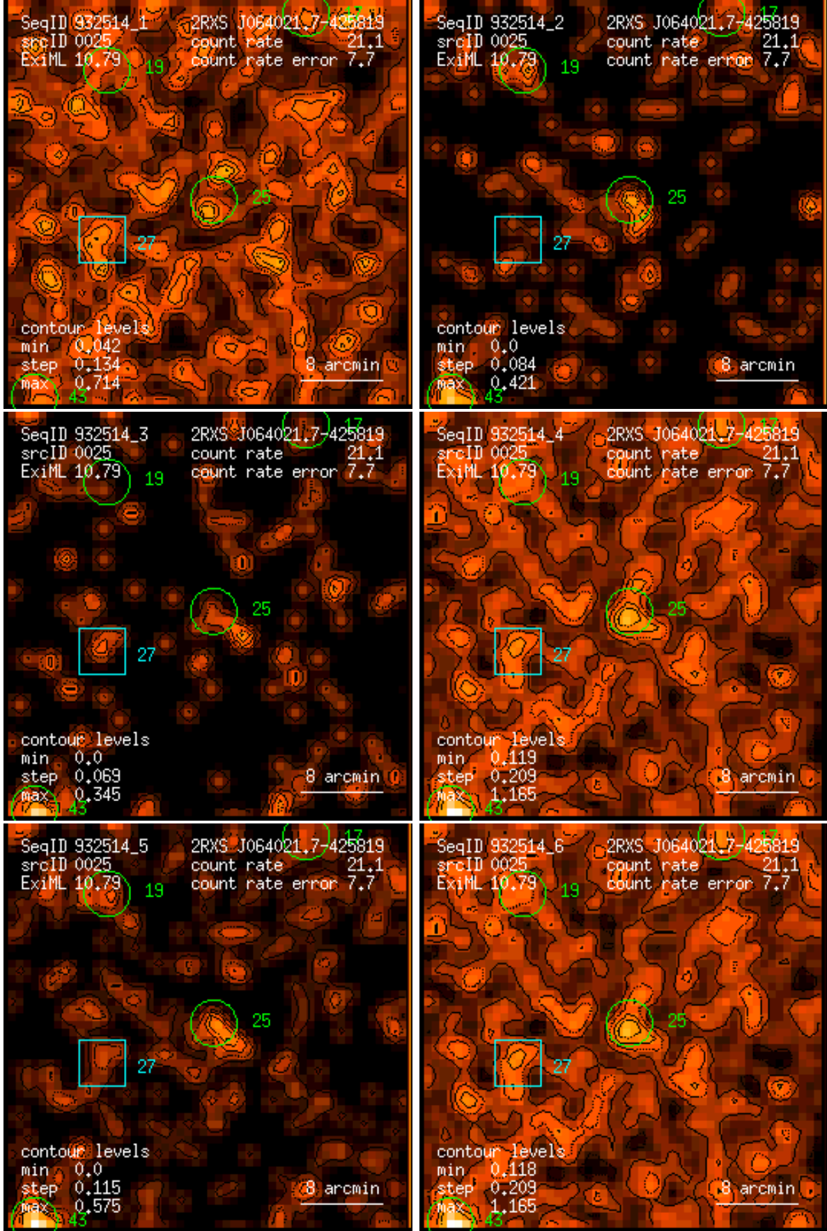
Figure 25: RASS 932514: detection 0025: band rate images, Gaussian filter: (1) PSPC channels 11 – 41, (2) 52 – 90, (3) 91 – 201, (4) 11 – 235, (5) 52 – 201, (6) 11 – 201. Broad band rates in counts/ks. Band rate contour levels in counts/ks/arcmin 2 .
