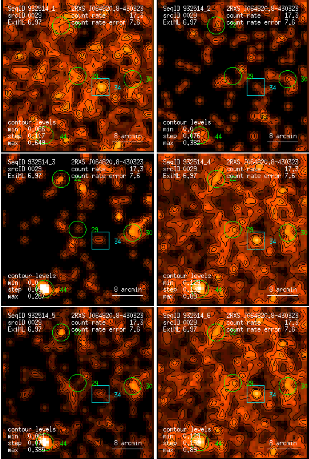
Figure 29: RASS 932514: detection 0029: band rate images, Gaussian filter: (1) PSPC channels 11 – 41, (2) 52 – 90, (3) 91 – 201, (4) 11 – 235, (5) 52 – 201, (6) 11 – 201. Broad band rates in counts/ks. Band rate contour levels in counts/ks/arcmin 2 .
