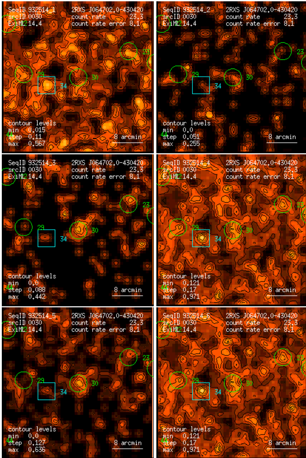
Figure 30: RASS 932514: detection 0030: band rate images, Gaussian filter: (1) PSPC channels 11 – 41, (2) 52 – 90, (3) 91 – 201, (4) 11 – 235, (5) 52 – 201, (6) 11 – 201. Broad band rates in counts/ks. Band rate contour levels in counts/ks/arcmin 2 .
