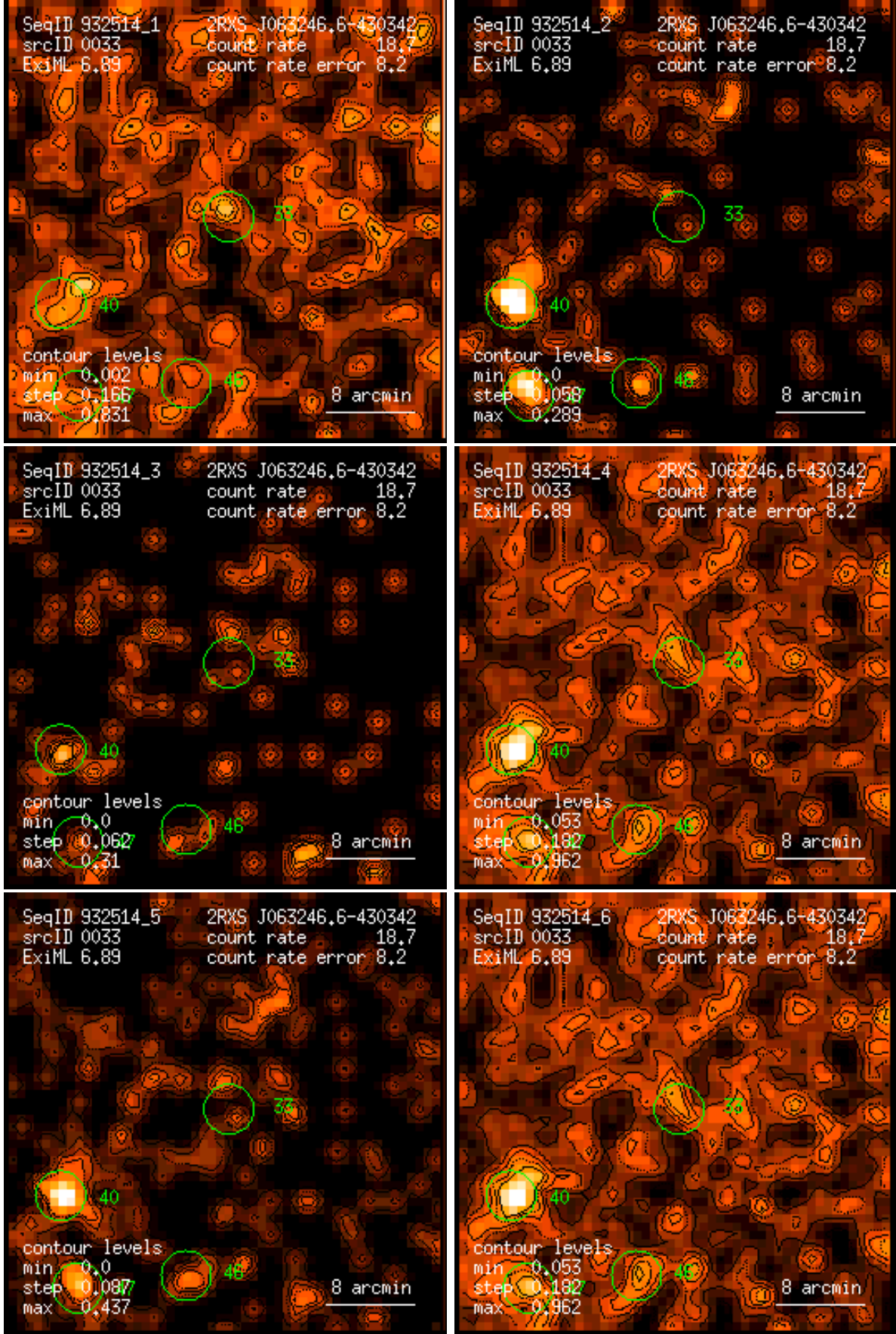
Figure 33: RASS 932514: detection 0033: band rate images, Gaussian filter: (1) PSPC channels 11 – 41, (2) 52 – 90, (3) 91 – 201, (4) 11 – 235, (5) 52 – 201, (6) 11 – 201. Broad band rates in counts/ks. Band rate contour levels in counts/ks/arcmin 2 .
