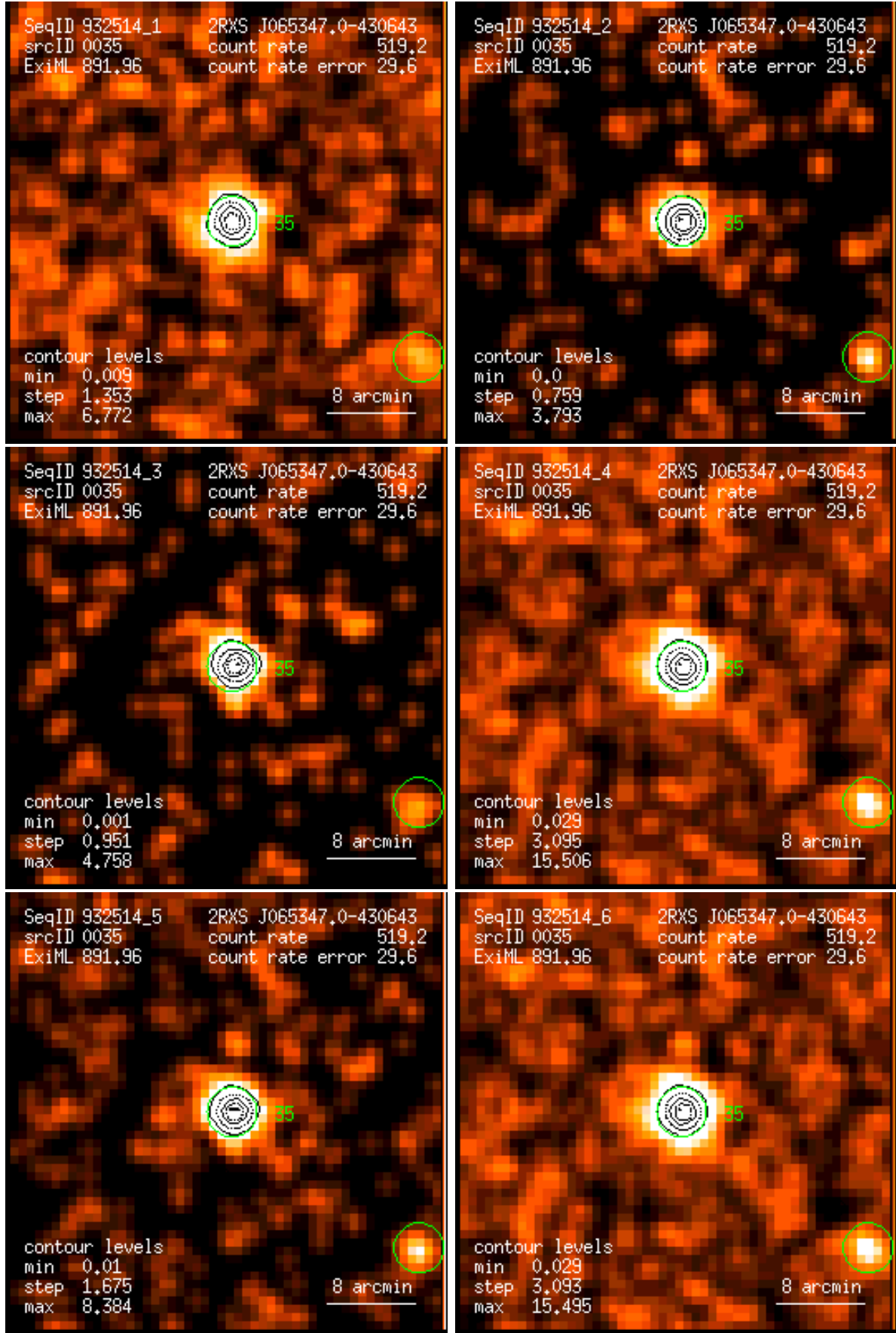
Figure 35: RASS 932514: detection 0035: band rate images, Gaussian filter: (1) PSPC channels 11 – 41, (2) 52 – 90, (3) 91 – 201, (4) 11 – 235, (5) 52 – 201, (6) 11 – 201. Broad band rates in counts/ks. Band rate contour levels in counts/ks/arcmin 2 .
