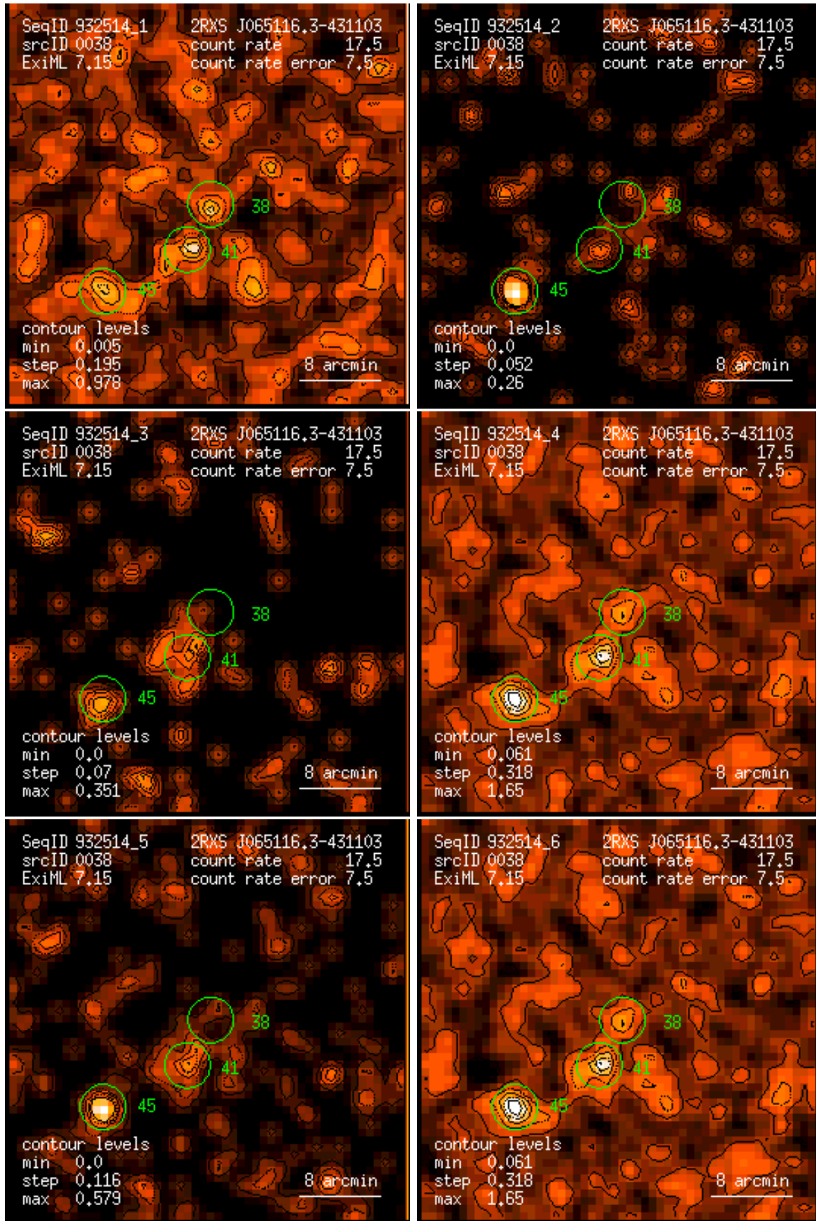
Figure 38: RASS 932514: detection 0038: band rate images, Gaussian filter: (1) PSPC channels 11 – 41, (2) 52 – 90, (3) 91 – 201, (4) 11 – 235, (5) 52 – 201, (6) 11 – 201. Broad band rates in counts/ks. Band rate contour levels in counts/ks/arcmin 2 .
