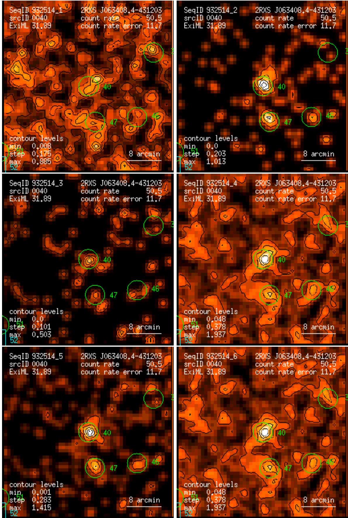
Figure 40: RASS 932514: detection 0040: band rate images, Gaussian filter: (1) PSPC channels 11 – 41, (2) 52 – 90, (3) 91 – 201, (4) 11 – 235, (5) 52 – 201, (6) 11 – 201. Broad band rates in counts/ks. Band rate contour levels in counts/ks/arcmin 2 .
