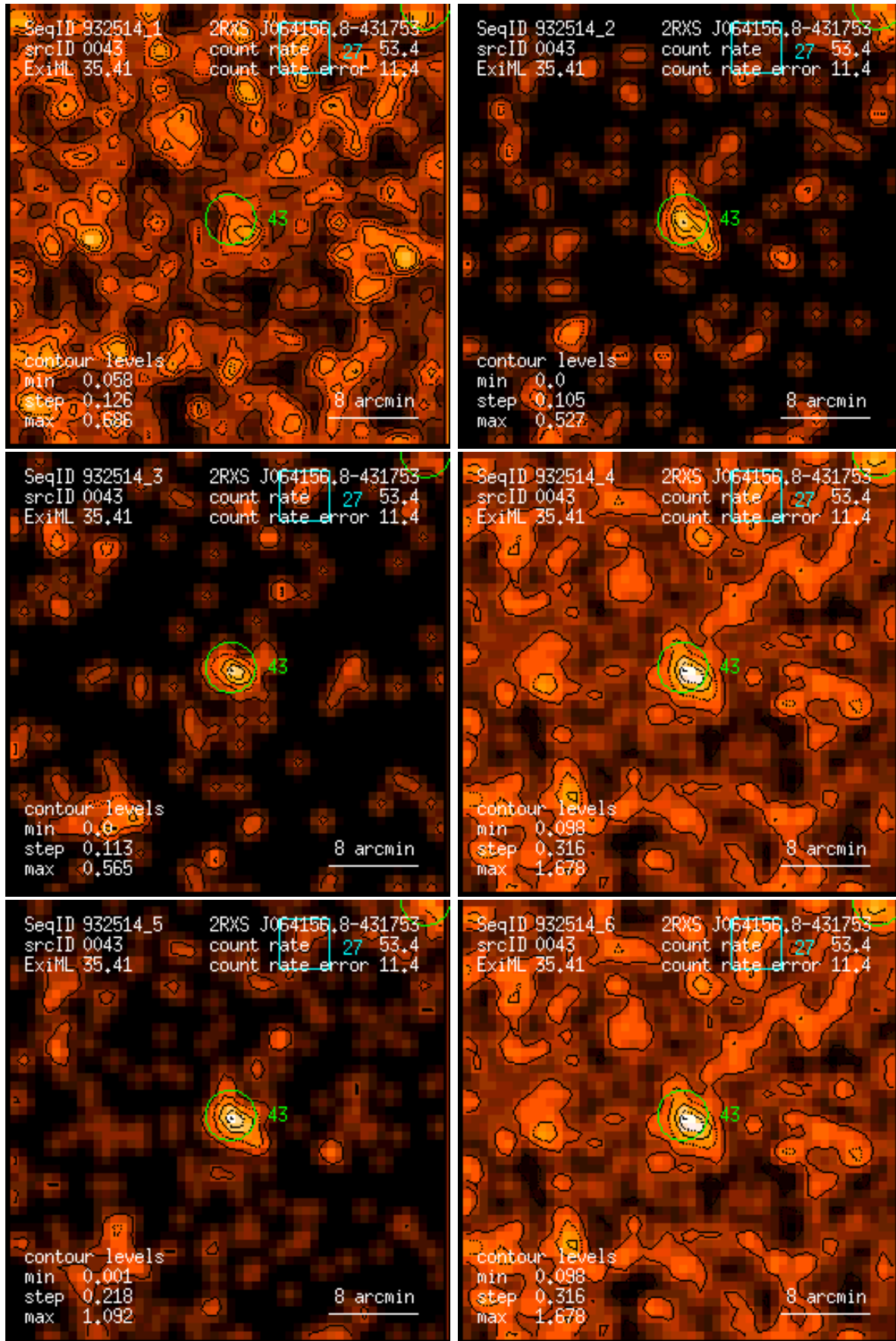
Figure 43: RASS 932514: detection 0043: band rate images, Gaussian filter: (1) PSPC channels 11 – 41, (2) 52 – 90, (3) 91 – 201, (4) 11 – 235, (5) 52 – 201, (6) 11 – 201. Broad band rates in counts/ks. Band rate contour levels in counts/ks/arcmin 2 .
