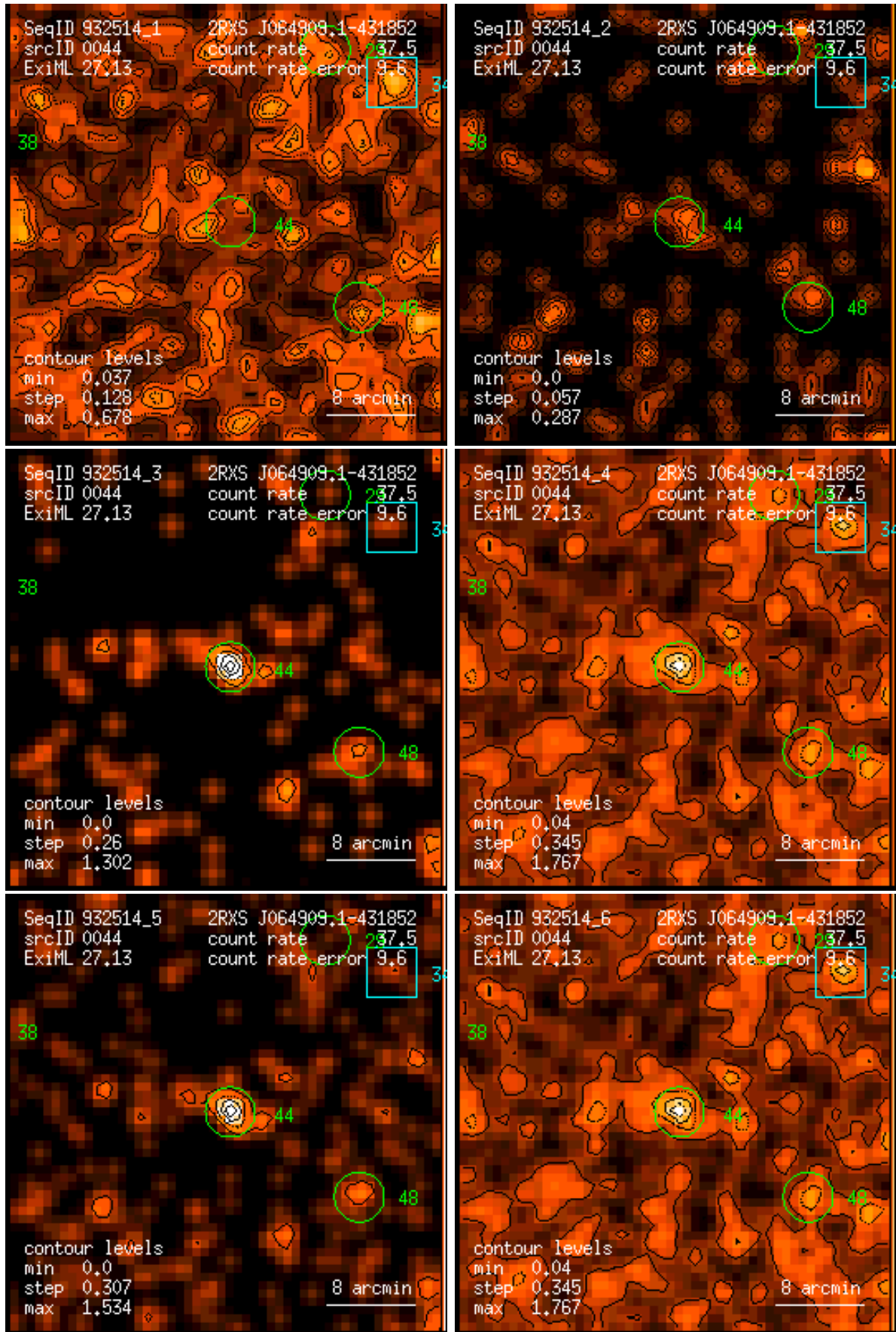
Figure 44: RASS 932514: detection 0044: band rate images, Gaussian filter: (1) PSPC channels 11 – 41, (2) 52 – 90, (3) 91 – 201, (4) 11 – 235, (5) 52 – 201, (6) 11 – 201. Broad band rates in counts/ks. Band rate contour levels in counts/ks/arcmin 2 .
