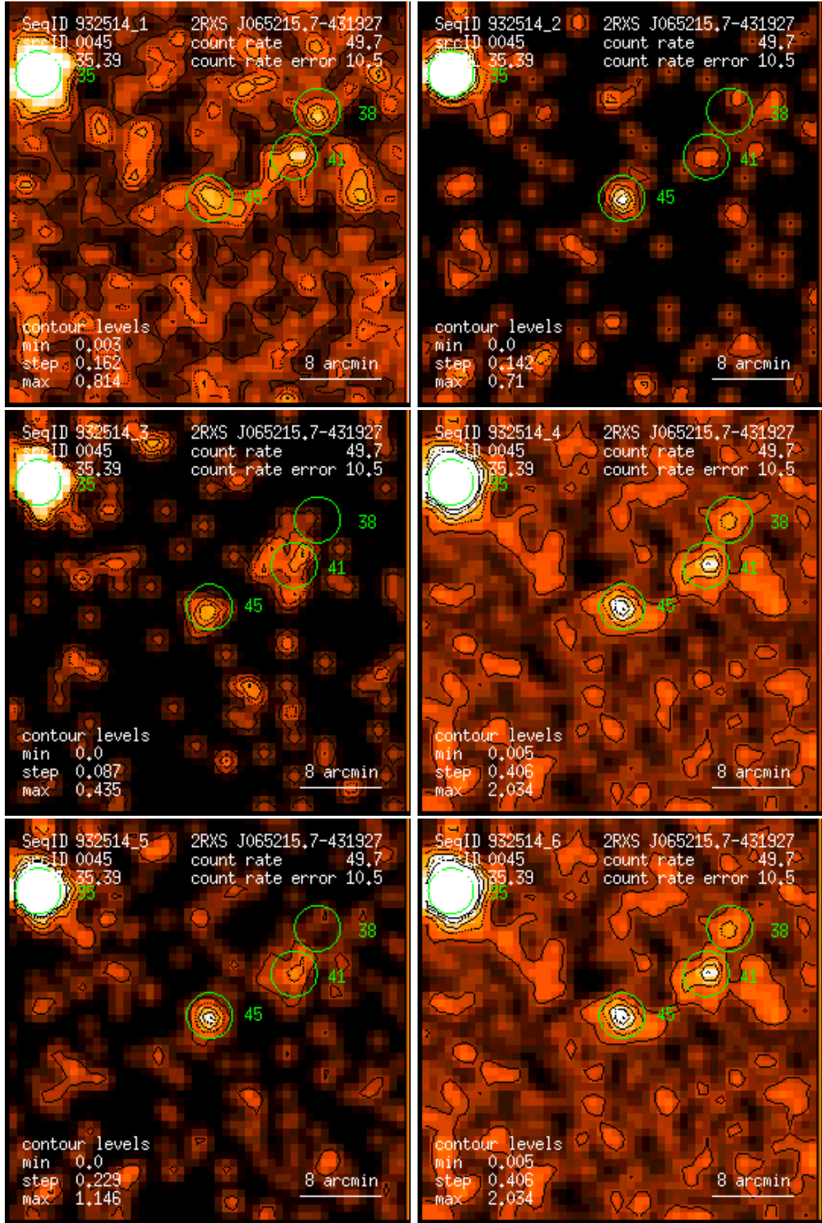
Figure 45: RASS 932514: detection 0045: band rate images, Gaussian filter: (1) PSPC channels 11 – 41, (2) 52 – 90, (3) 91 – 201, (4) 11 – 235, (5) 52 – 201, (6) 11 – 201. Broad band rates in counts/ks. Band rate contour levels in counts/ks/arcmin 2 .
