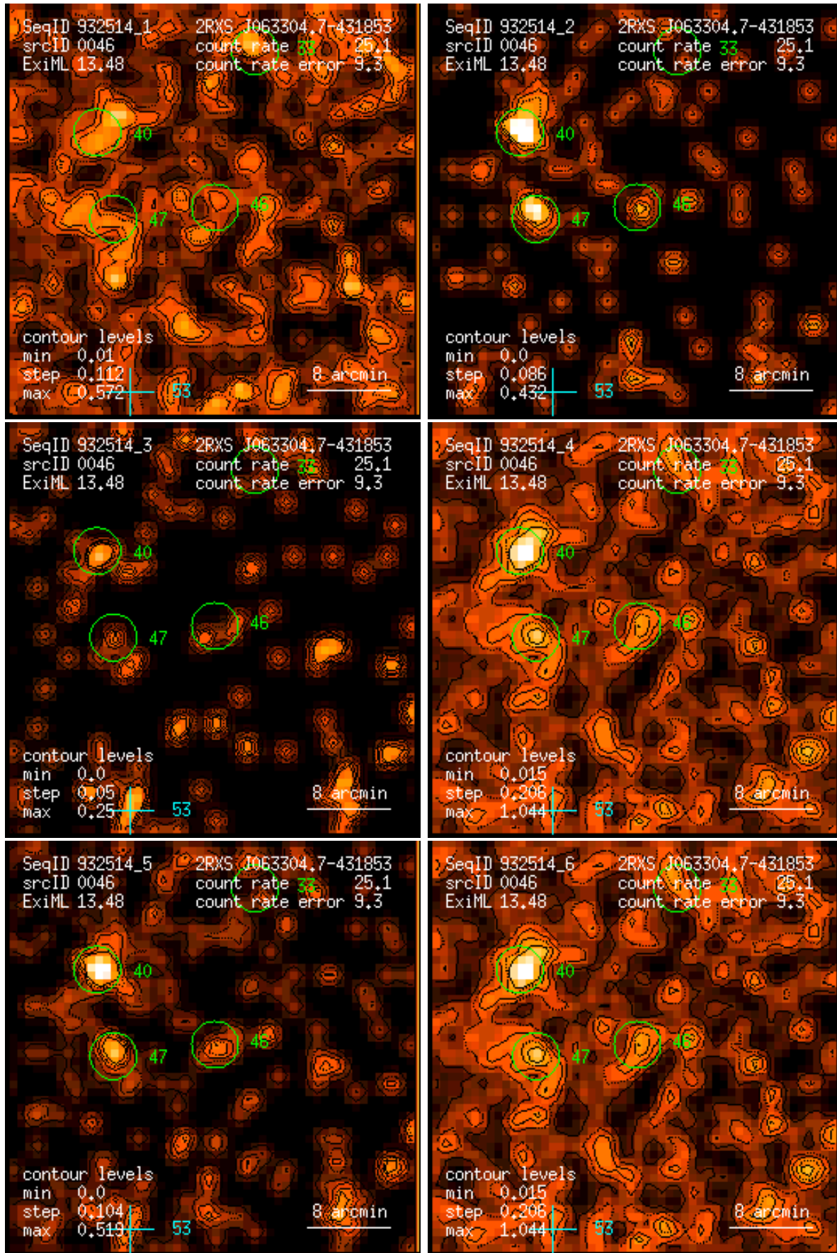
Figure 46: RASS 932514: detection 0046: band rate images, Gaussian filter: (1) PSPC channels 11 – 41, (2) 52 – 90, (3) 91 – 201, (4) 11 – 235, (5) 52 – 201, (6) 11 – 201. Broad band rates in counts/ks. Band rate contour levels in counts/ks/arcmin 2 .
