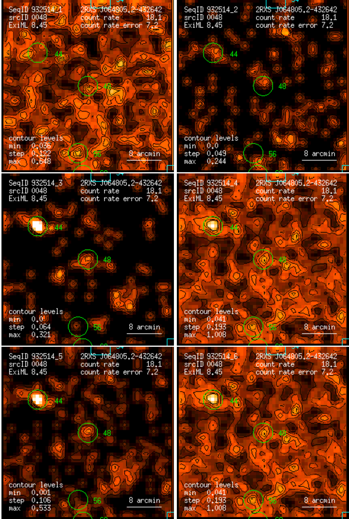
Figure 48: RASS 932514: detection 0048: band rate images, Gaussian filter: (1) PSPC channels 11 – 41, (2) 52 – 90, (3) 91 – 201, (4) 11 – 235, (5) 52 – 201, (6) 11 – 201. Broad band rates in counts/ks. Band rate contour levels in counts/ks/arcmin 2 .
