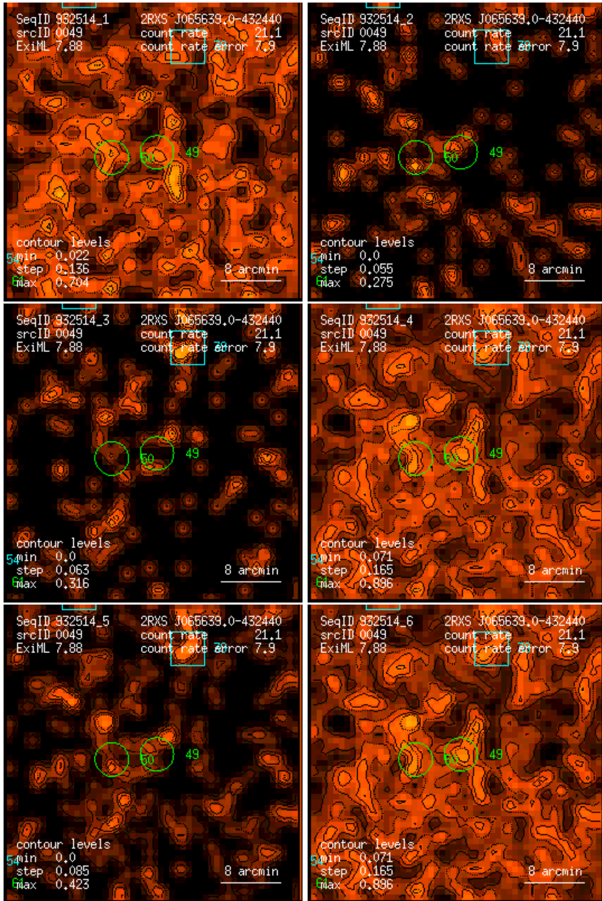
Figure 49: RASS 932514: detection 0049: band rate images, Gaussian filter: (1) PSPC channels 11 – 41, (2) 52 – 90, (3) 91 – 201, (4) 11 – 235, (5) 52 – 201, (6) 11 – 201. Broad band rates in counts/ks. Band rate contour levels in counts/ks/arcmin 2 .
