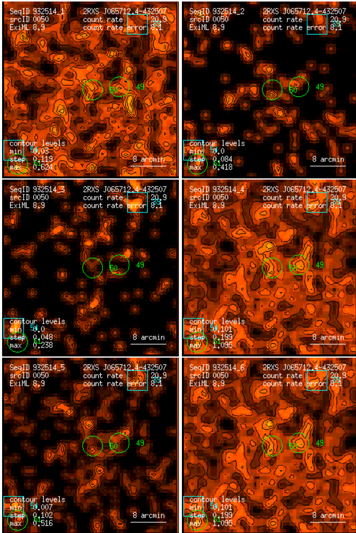
Figure 50: RASS 932514: detection 0050: band rate images, Gaussian filter: (1) PSPC channels 11 – 41, (2) 52 – 90, (3) 91 – 201, (4) 11 – 235, (5) 52 – 201, (6) 11 – 201. Broad band rates in counts/ks. Band rate contour levels in counts/ks/arcmin 2 .
