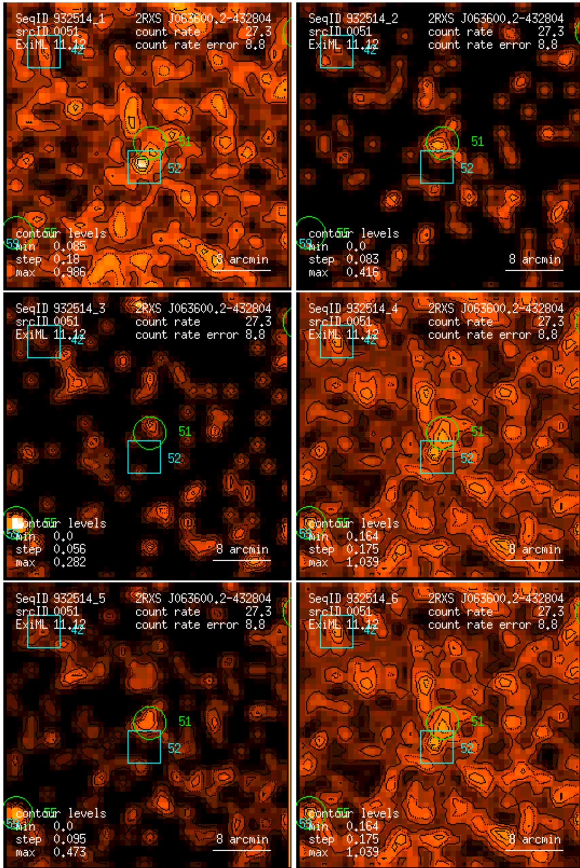
Figure 51: RASS 932514: detection 0051: band rate images, Gaussian filter: (1) PSPC channels 11 – 41, (2) 52 – 90, (3) 91 – 201, (4) 11 – 235, (5) 52 – 201, (6) 11 – 201. Broad band rates in counts/ks. Band rate contour levels in counts/ks/arcmin 2 .
