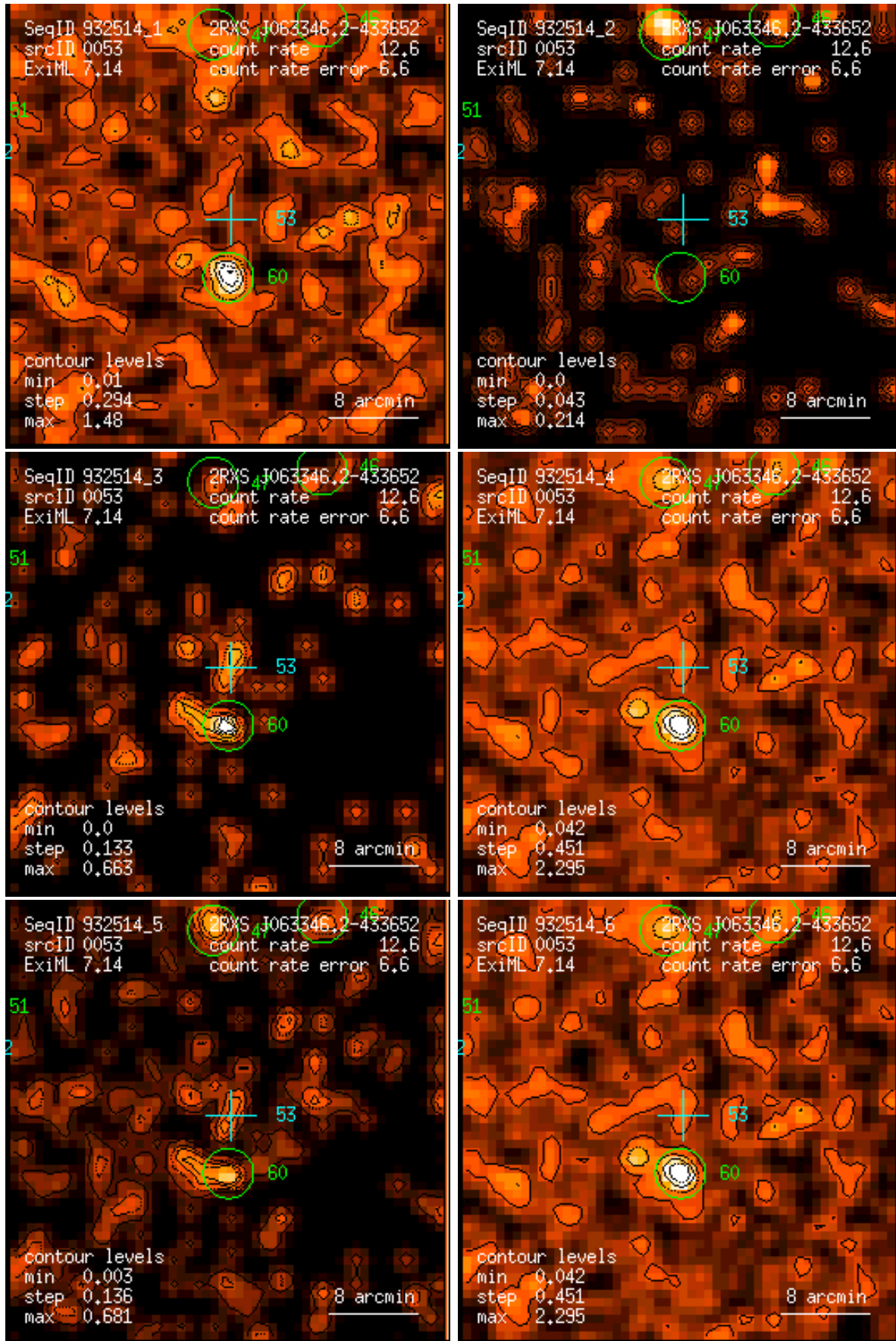
Figure 53: RASS 932514: detection 0053: band rate images, Gaussian filter: (1) PSPC channels 11 – 41, (2) 52 – 90, (3) 91 – 201, (4) 11 – 235, (5) 52 – 201, (6) 11 – 201. Broad band rates in counts/ks. Band rate contour levels in counts/ks/arcmin 2 .
