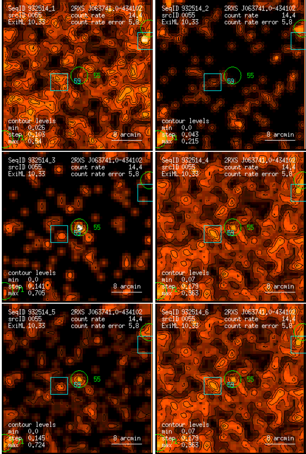
Figure 55: RASS 932514: detection 0055: band rate images, Gaussian filter: (1) PSPC channels 11 – 41, (2) 52 – 90, (3) 91 – 201, (4) 11 – 235, (5) 52 – 201, (6) 11 – 201. Broad band rates in counts/ks. Band rate contour levels in counts/ks/arcmin 2 .
