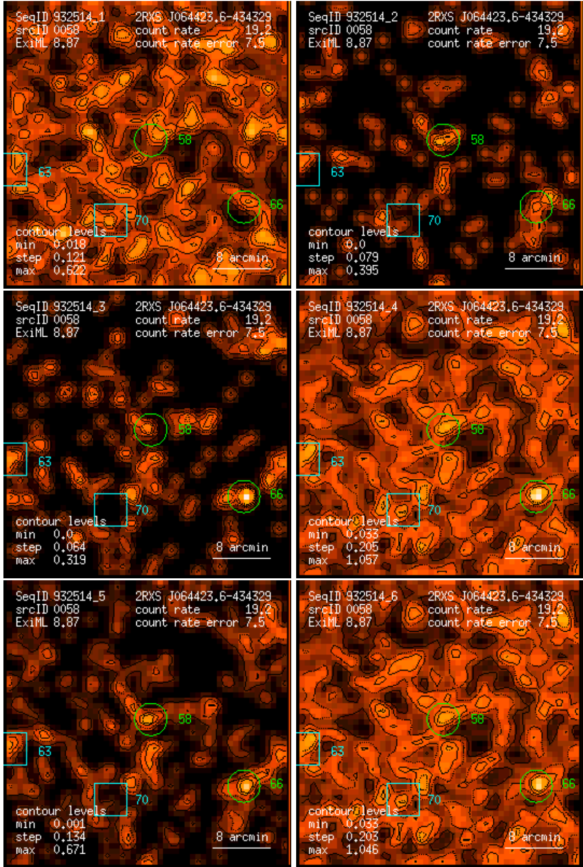
Figure 58: RASS 932514: detection 0058: band rate images, Gaussian filter: (1) PSPC channels 11 – 41, (2) 52 – 90, (3) 91 – 201, (4) 11 – 235, (5) 52 – 201, (6) 11 – 201. Broad band rates in counts/ks. Band rate contour levels in counts/ks/arcmin 2 .
