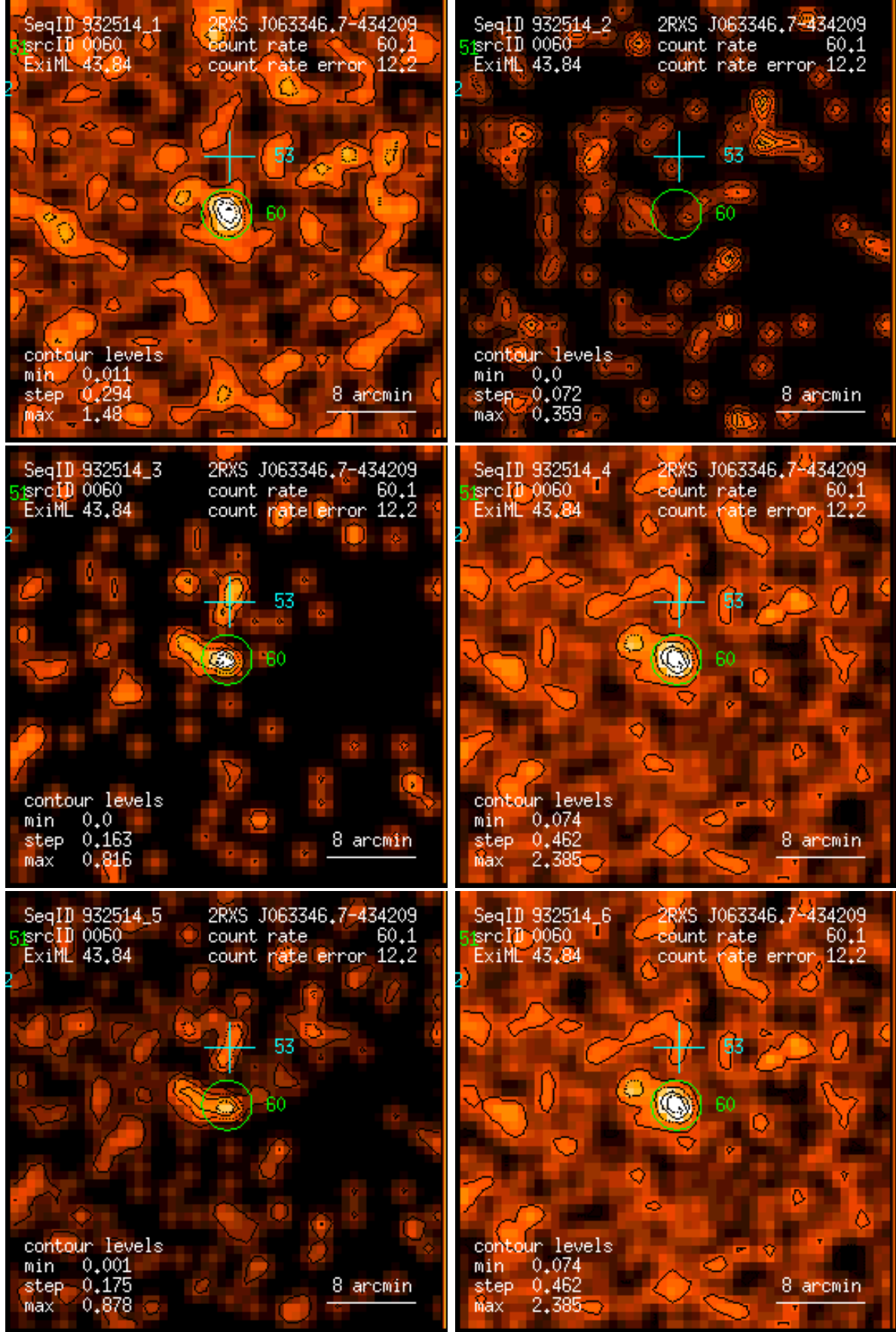
Figure 60: RASS 932514: detection 0060: band rate images, Gaussian filter: (1) PSPC channels 11 – 41, (2) 52 – 90, (3) 91 – 201, (4) 11 – 235, (5) 52 – 201, (6) 11 – 201. Broad band rates in counts/ks. Band rate contour levels in counts/ks/arcmin 2 .
