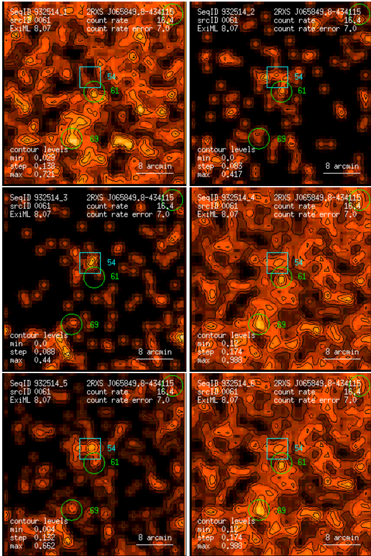
Figure 61: RASS 932514: detection 0061: band rate images, Gaussian filter: (1) PSPC channels 11 – 41, (2) 52 – 90, (3) 91 – 201, (4) 11 – 235, (5) 52 – 201, (6) 11 – 201. Broad band rates in counts/ks. Band rate contour levels in counts/ks/arcmin 2 .
