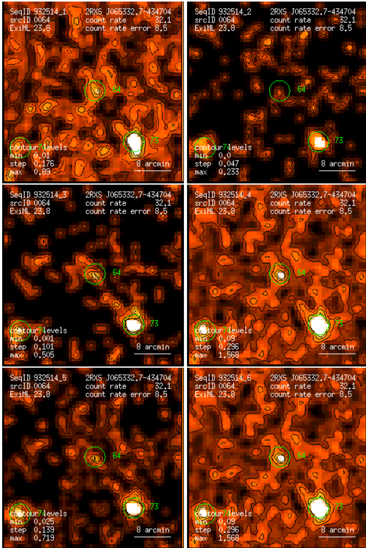
Figure 64: RASS 932514: detection 0064: band rate images, Gaussian filter: (1) PSPC channels 11 – 41, (2) 52 – 90, (3) 91 – 201, (4) 11 – 235, (5) 52 – 201, (6) 11 – 201. Broad band rates in counts/ks. Band rate contour levels in counts/ks/arcmin 2 .
