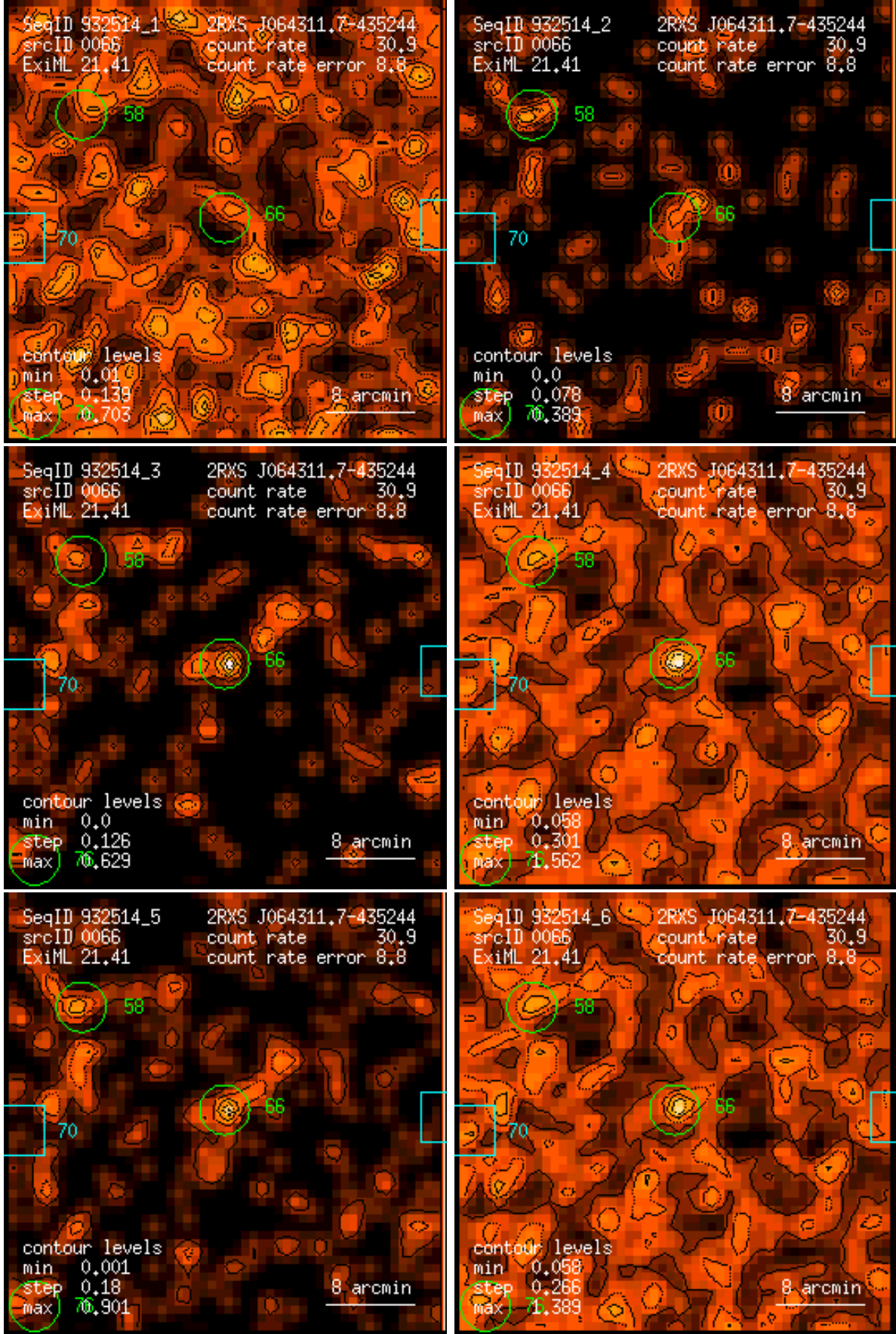
Figure 66: RASS 932514: detection 0066: band rate images, Gaussian filter: (1) PSPC channels 11 – 41, (2) 52 – 90, (3) 91 – 201, (4) 11 – 235, (5) 52 – 201, (6) 11 – 201. Broad band rates in counts/ks. Band rate contour levels in counts/ks/arcmin 2 .
