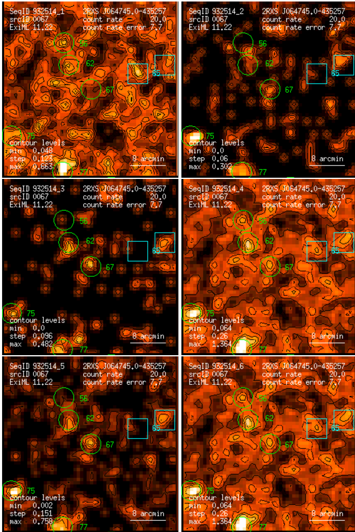
Figure 67: RASS 932514: detection 0067: band rate images, Gaussian filter: (1) PSPC channels 11 – 41, (2) 52 – 90, (3) 91 – 201, (4) 11 – 235, (5) 52 – 201, (6) 11 – 201. Broad band rates in counts/ks. Band rate contour levels in counts/ks/arcmin 2 .
