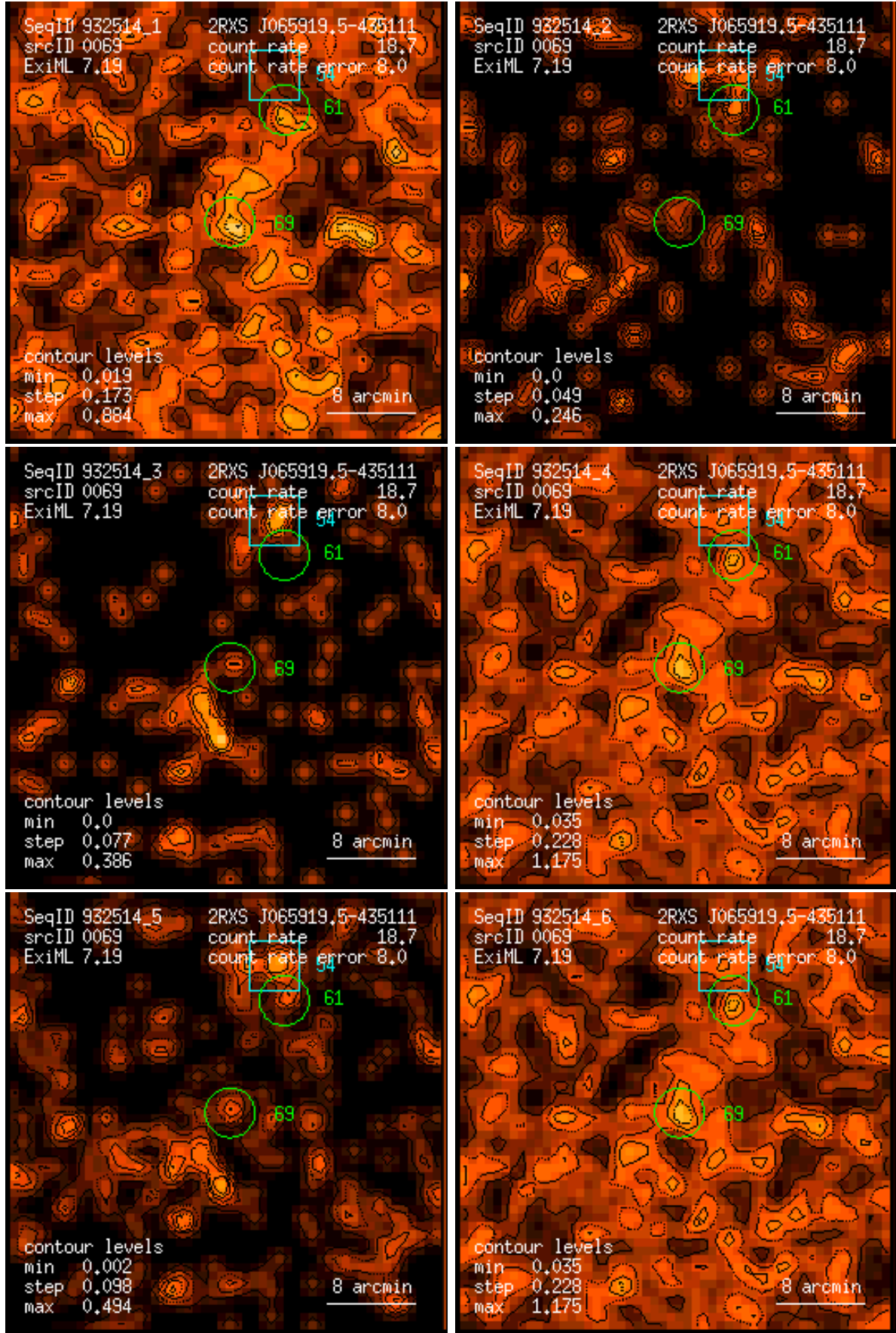
Figure 69: RASS 932514: detection 0069: band rate images, Gaussian filter: (1) PSPC channels 11 – 41, (2) 52 – 90, (3) 91 – 201, (4) 11 – 235, (5) 52 – 201, (6) 11 – 201. Broad band rates in counts/ks. Band rate contour levels in counts/ks/arcmin 2 .
