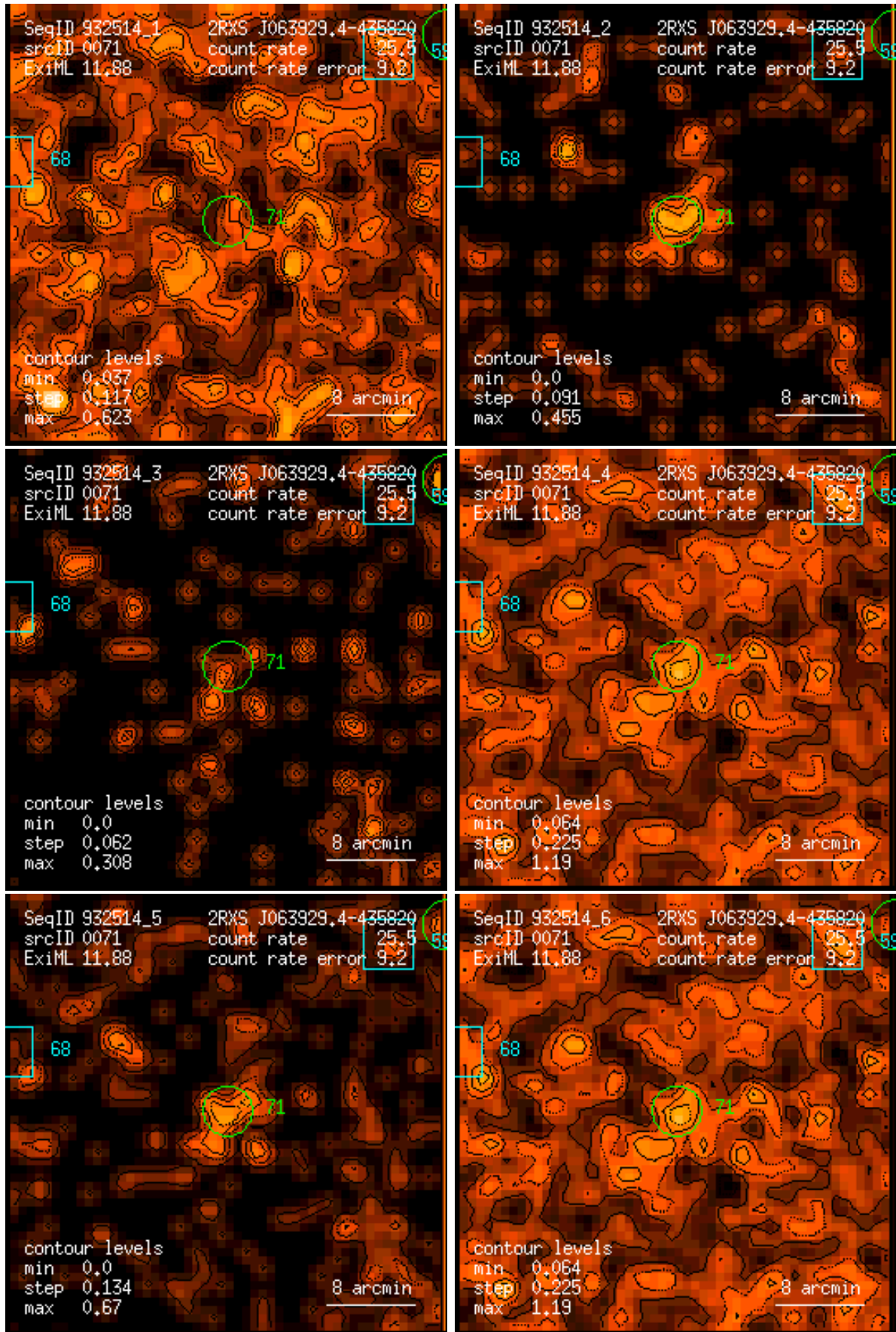
Figure 71: RASS 932514: detection 0071: band rate images, Gaussian filter: (1) PSPC channels 11 – 41, (2) 52 – 90, (3) 91 – 201, (4) 11 – 235, (5) 52 – 201, (6) 11 – 201. Broad band rates in counts/ks. Band rate contour levels in counts/ks/arcmin 2 .
