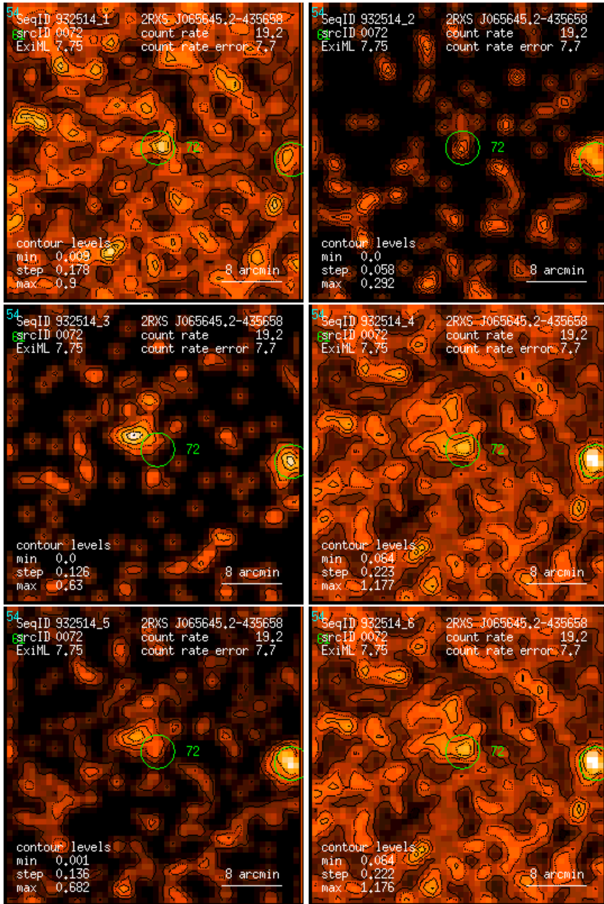
Figure 72: RASS 932514: detection 0072: band rate images, Gaussian filter: (1) PSPC channels 11 – 41, (2) 52 – 90, (3) 91 – 201, (4) 11 – 235, (5) 52 – 201, (6) 11 – 201. Broad band rates in counts/ks. Band rate contour levels in counts/ks/arcmin 2 .
