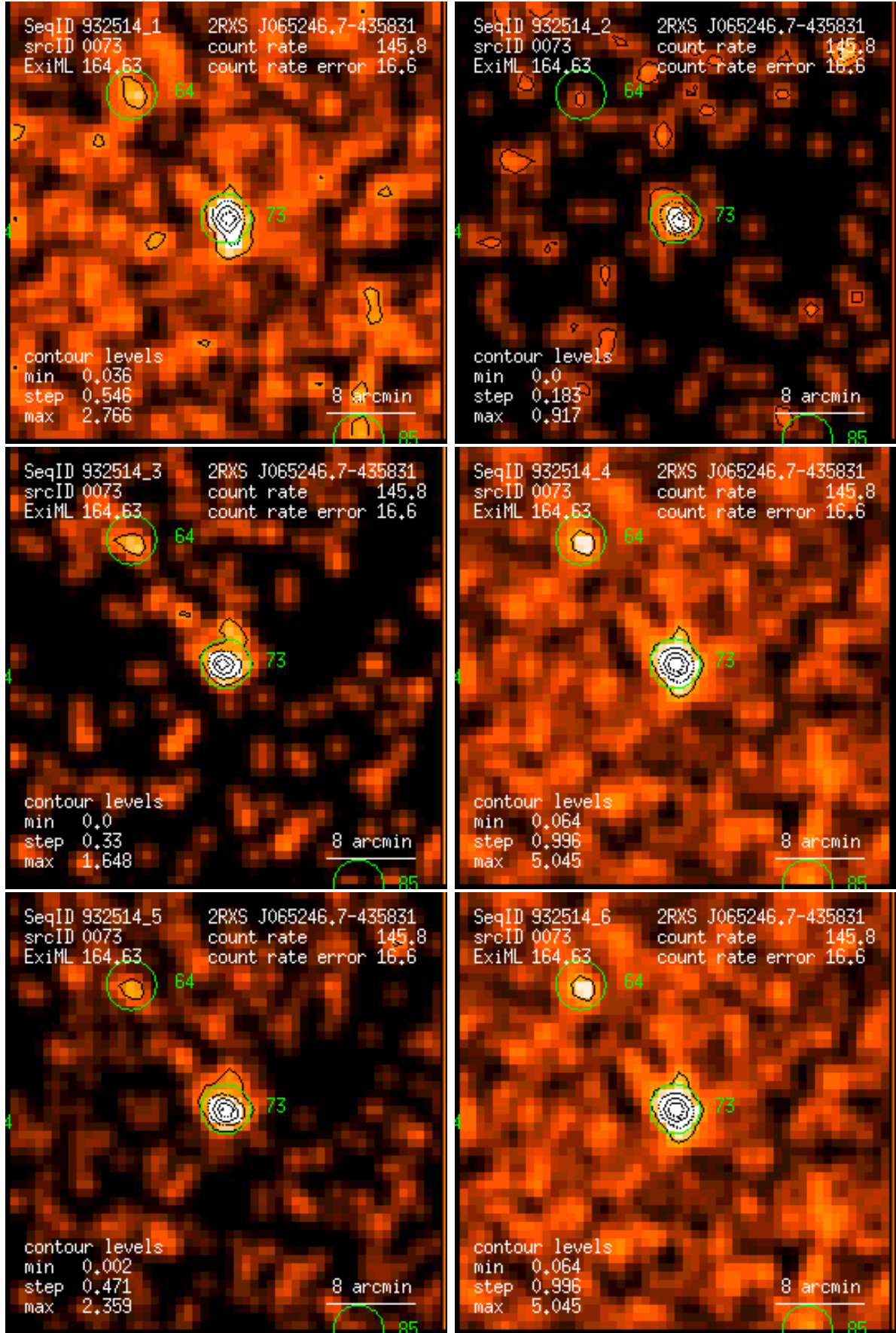
Figure 73: RASS 932514: detection 0073: band rate images, Gaussian filter: (1) PSPC channels 11 – 41, (2) 52 – 90, (3) 91 – 201, (4) 11 – 235, (5) 52 – 201, (6) 11 – 201. Broad band rates in counts/ks. Band rate contour levels in counts/ks/arcmin 2 .
