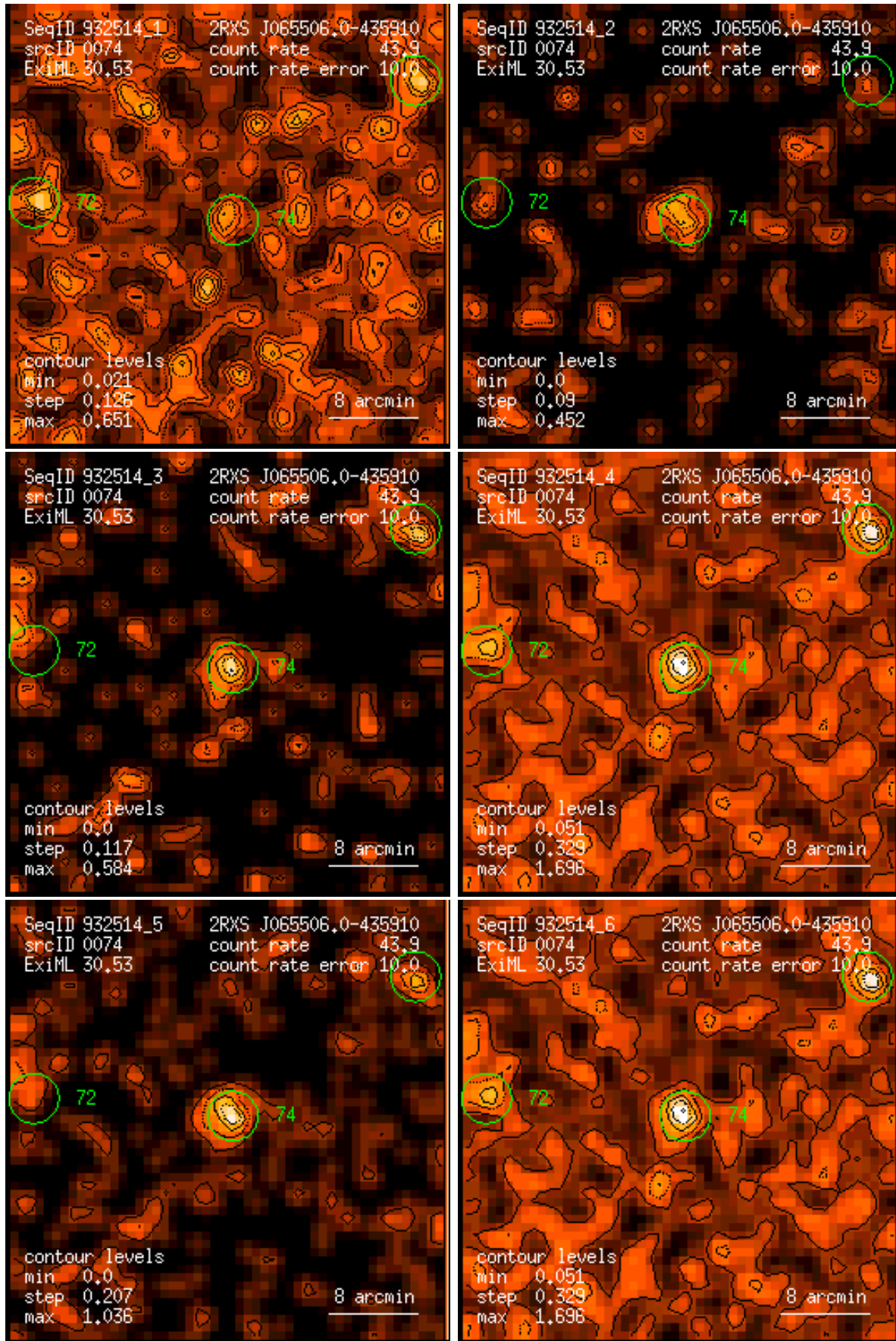
Figure 74: RASS 932514: detection 0074: band rate images, Gaussian filter: (1) PSPC channels 11 – 41, (2) 52 – 90, (3) 91 – 201, (4) 11 – 235, (5) 52 – 201, (6) 11 – 201. Broad band rates in counts/ks. Band rate contour levels in counts/ks/arcmin 2 .
