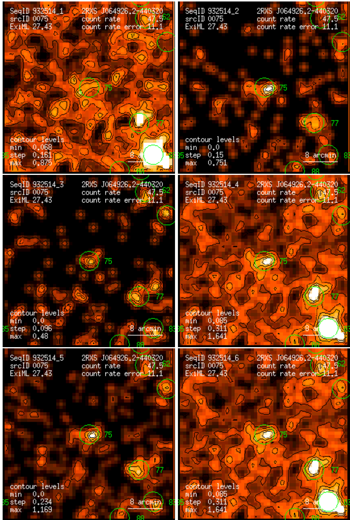
Figure 75: RASS 932514: detection 0075: band rate images, Gaussian filter: (1) PSPC channels 11 – 41, (2) 52 – 90, (3) 91 – 201, (4) 11 – 235, (5) 52 – 201, (6) 11 – 201. Broad band rates in counts/ks. Band rate contour levels in counts/ks/arcmin 2 .
