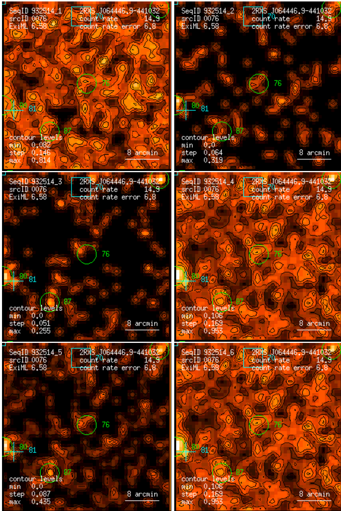
Figure 76: RASS 932514: detection 0076: band rate images, Gaussian filter: (1) PSPC channels 11 – 41, (2) 52 – 90, (3) 91 – 201, (4) 11 – 235, (5) 52 – 201, (6) 11 – 201. Broad band rates in counts/ks. Band rate contour levels in counts/ks/arcmin 2 .
