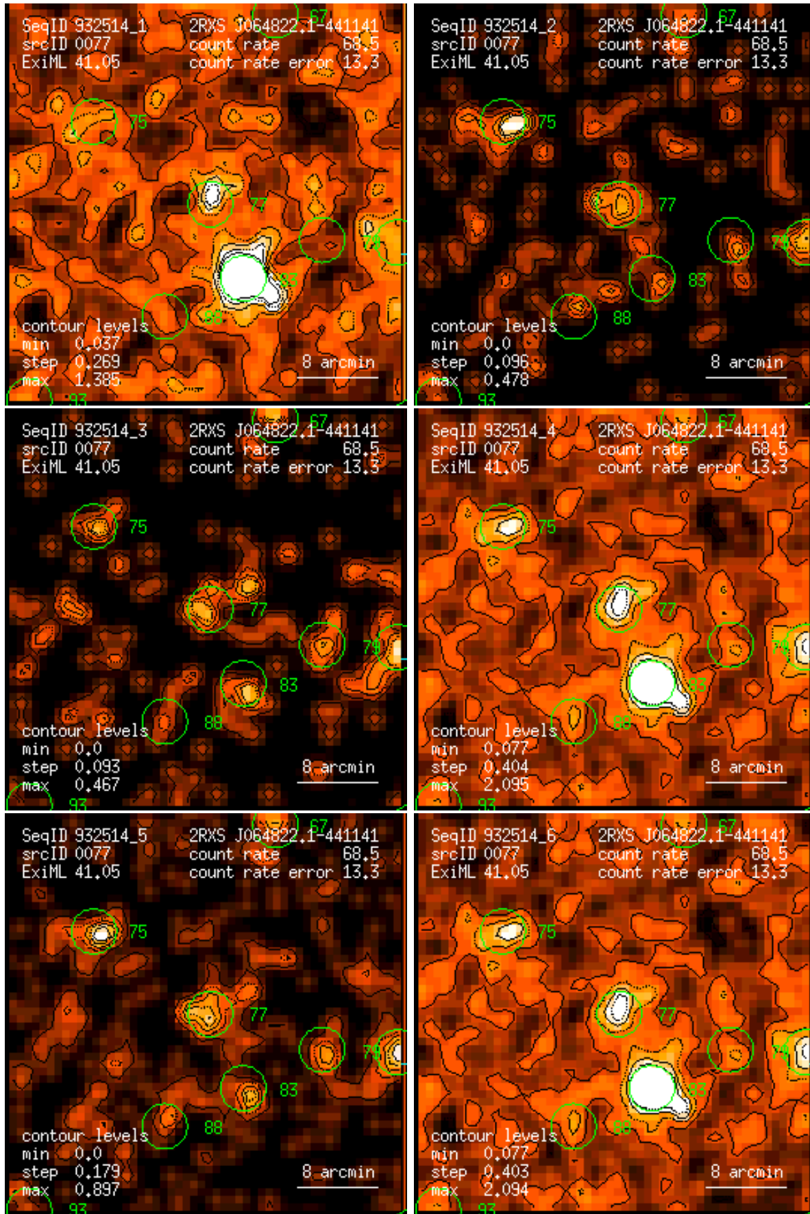
Figure 77: RASS 932514: detection 0077: band rate images, Gaussian filter: (1) PSPC channels 11 – 41, (2) 52 – 90, (3) 91 – 201, (4) 11 – 235, (5) 52 – 201, (6) 11 – 201. Broad band rates in counts/ks. Band rate contour levels in counts/ks/arcmin 2 .
