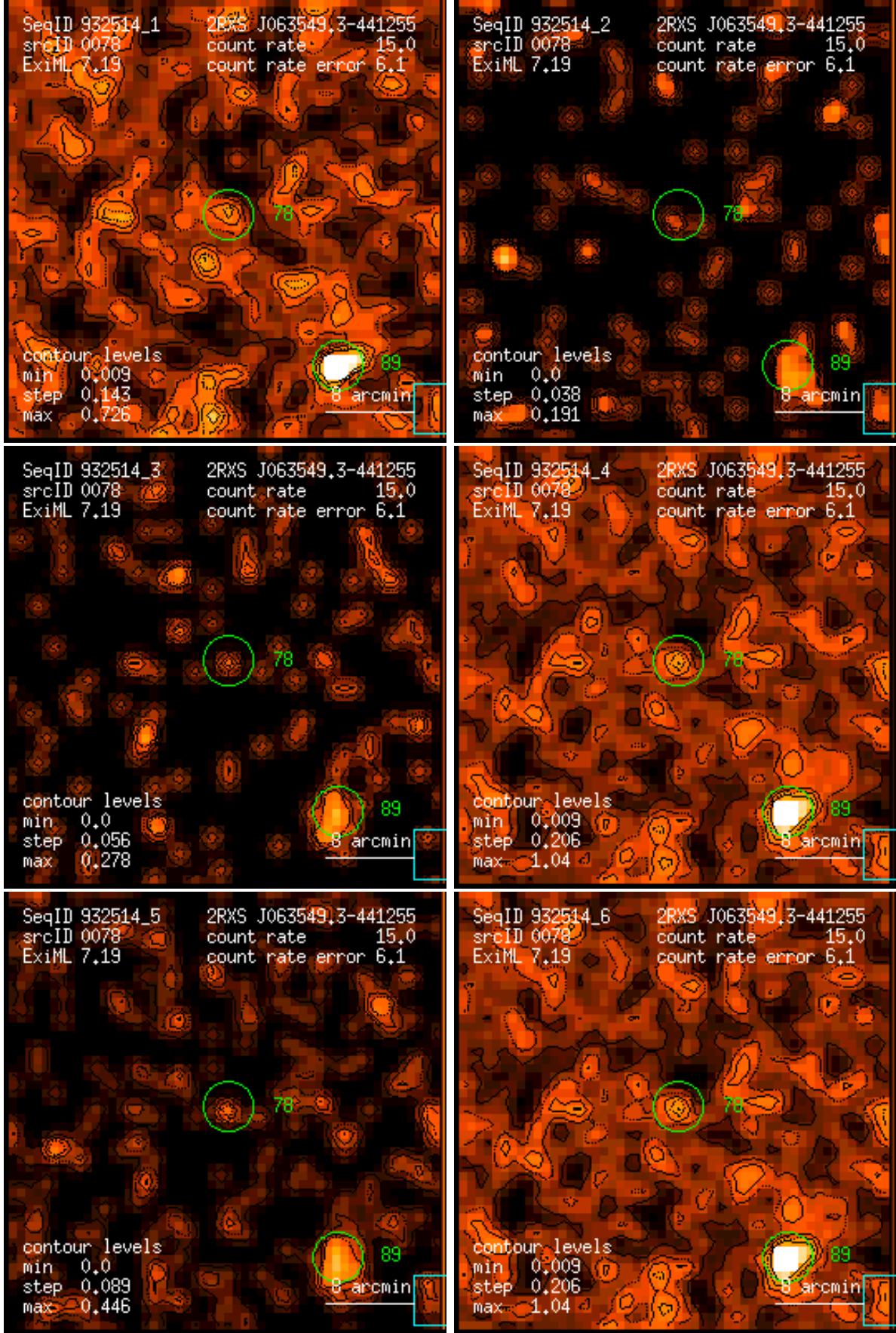
Figure 78: RASS 932514: detection 0078: band rate images, Gaussian filter: (1) PSPC channels 11 – 41, (2) 52 – 90, (3) 91 – 201, (4) 11 – 235, (5) 52 – 201, (6) 11 – 201. Broad band rates in counts/ks. Band rate contour levels in counts/ks/arcmin 2 .
