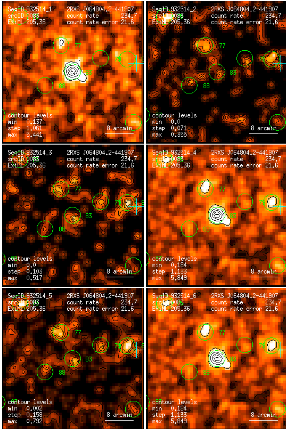
Figure 83: RASS 932514: detection 0083: band rate images, Gaussian filter: (1) PSPC channels 11 – 41, (2) 52 – 90, (3) 91 – 201, (4) 11 – 235, (5) 52 – 201, (6) 11 – 201. Broad band rates in counts/ks. Band rate contour levels in counts/ks/arcmin 2 .
