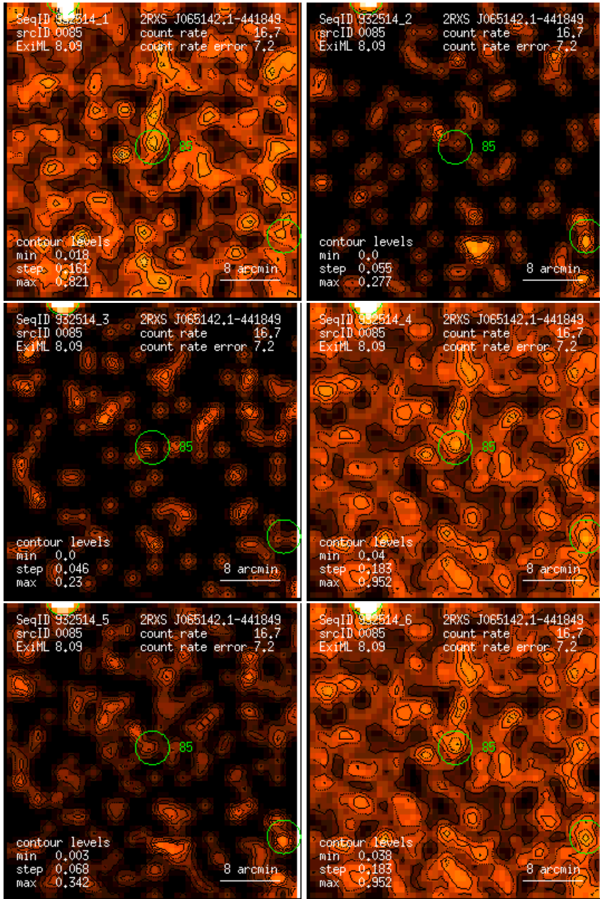
Figure 85: RASS 932514: detection 0085: band rate images, Gaussian filter: (1) PSPC channels 11 – 41, (2) 52 – 90, (3) 91 – 201, (4) 11 – 235, (5) 52 – 201, (6) 11 – 201. Broad band rates in counts/ks. Band rate contour levels in counts/ks/arcmin 2 .
