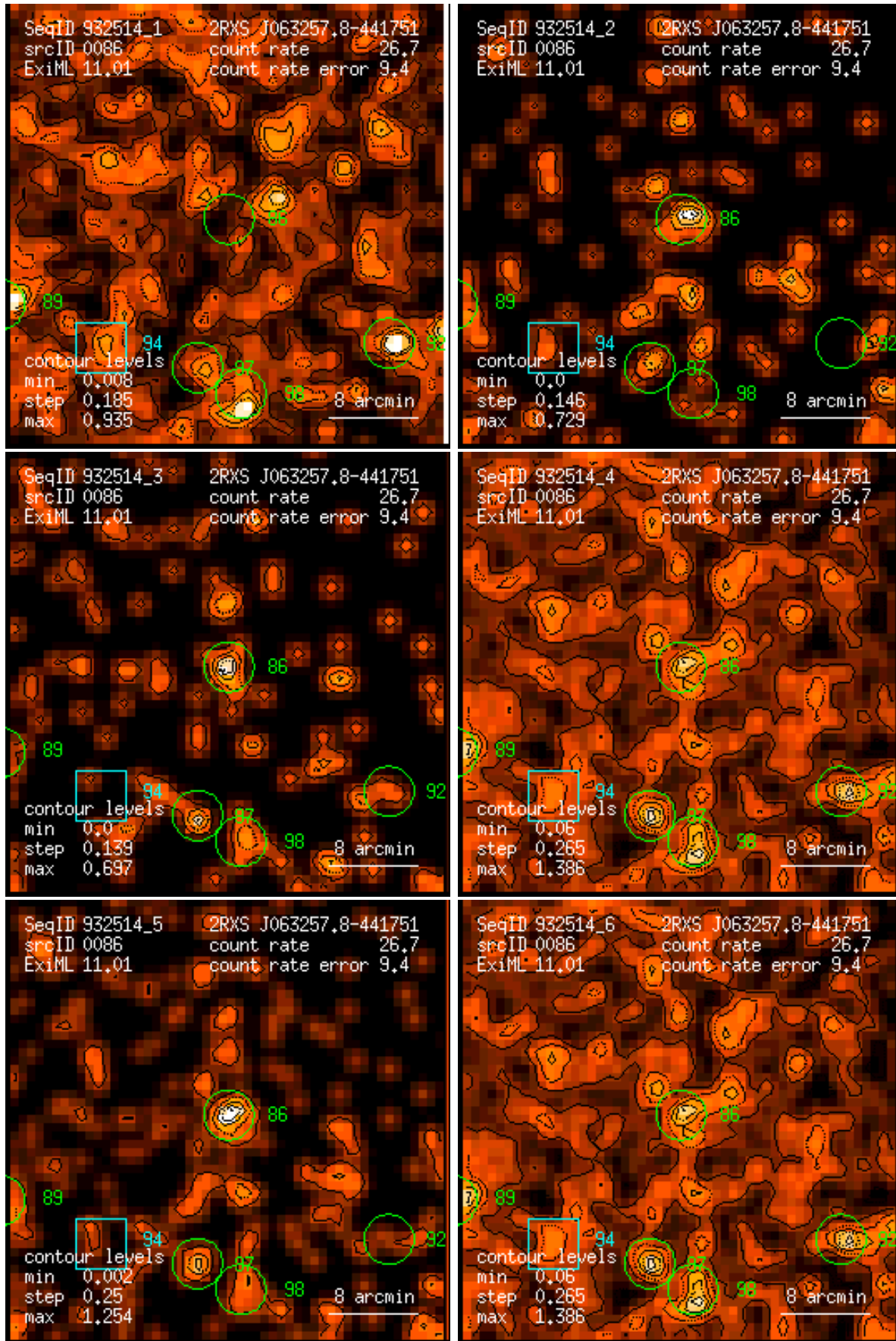
Figure 86: RASS 932514: detection 0086: band rate images, Gaussian filter: (1) PSPC channels 11 – 41, (2) 52 – 90, (3) 91 – 201, (4) 11 – 235, (5) 52 – 201, (6) 11 – 201. Broad band rates in counts/ks. Band rate contour levels in counts/ks/arcmin 2 .
