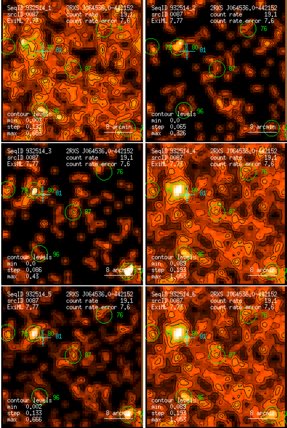
Figure 87: RASS 932514: detection 0087: band rate images, Gaussian filter: (1) PSPC channels 11 – 41, (2) 52 – 90, (3) 91 – 201, (4) 11 – 235, (5) 52 – 201, (6) 11 – 201. Broad band rates in counts/ks. Band rate contour levels in counts/ks/arcmin 2 .
