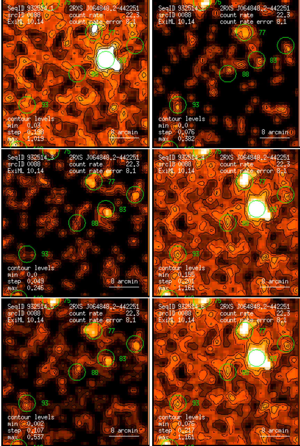
Figure 88: RASS 932514: detection 0088: band rate images, Gaussian filter: (1) PSPC channels 11 – 41, (2) 52 – 90, (3) 91 – 201, (4) 11 – 235, (5) 52 – 201, (6) 11 – 201. Broad band rates in counts/ks. Band rate contour levels in counts/ks/arcmin 2 .
