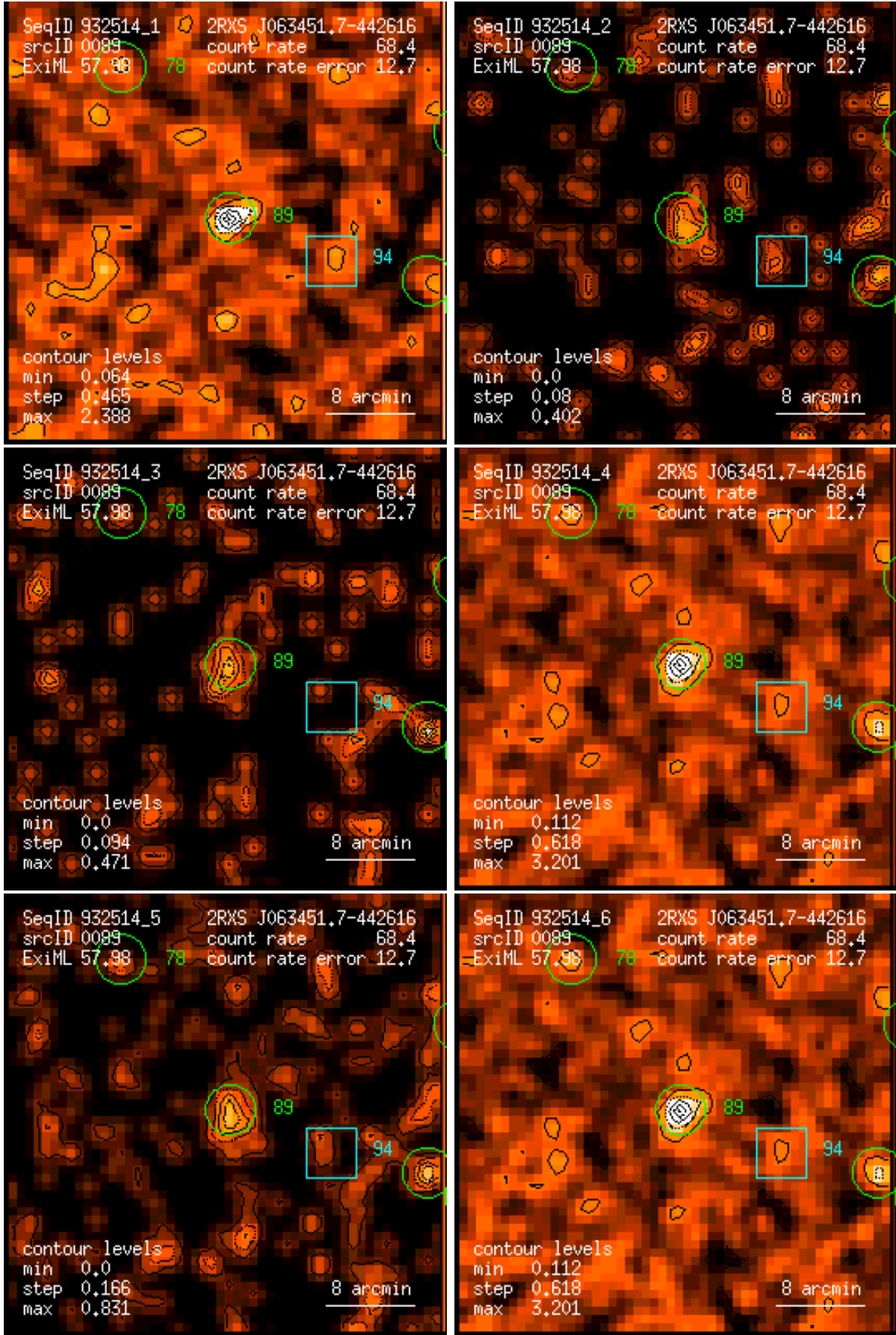
Figure 89: RASS 932514: detection 0089: band rate images, Gaussian filter: (1) PSPC channels 11 – 41, (2) 52 – 90, (3) 91 – 201, (4) 11 – 235, (5) 52 – 201, (6) 11 – 201. Broad band rates in counts/ks. Band rate contour levels in counts/ks/arcmin 2 .
