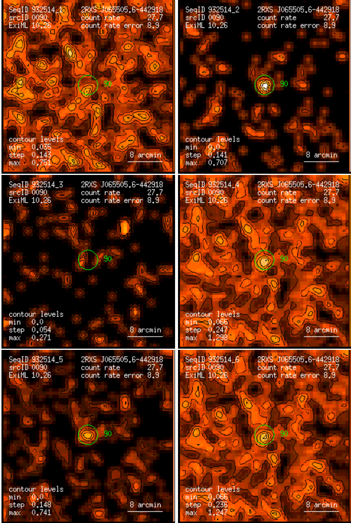
Figure 90: RASS 932514: detection 0090: band rate images, Gaussian filter: (1) PSPC channels 11 – 41, (2) 52 – 90, (3) 91 – 201, (4) 11 – 235, (5) 52 – 201, (6) 11 – 201. Broad band rates in counts/ks. Band rate contour levels in counts/ks/arcmin 2 .
